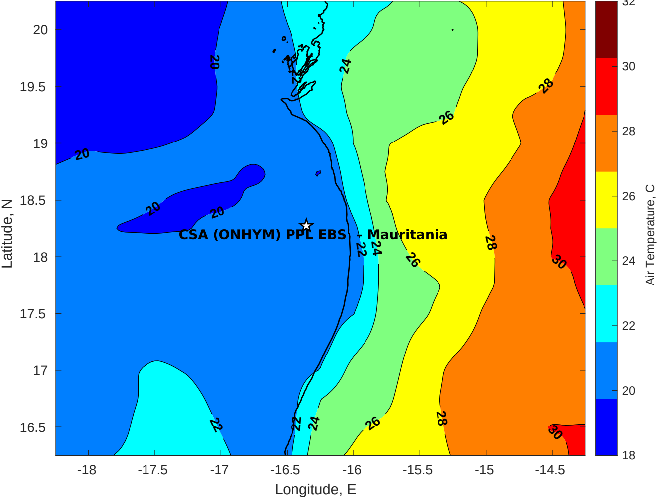
Air Temperature (C) for CSA (ONHYM) PPL EBS - Mauritania at 19-Apr-2025
