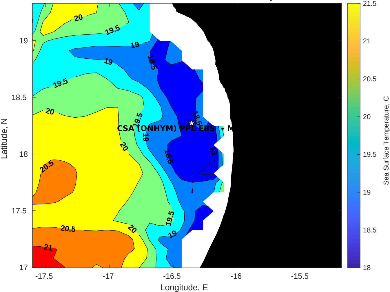
SST for CSA (ONHYM) PPL EBS - Mauritania at 18-Apr-2025 00:00:00
