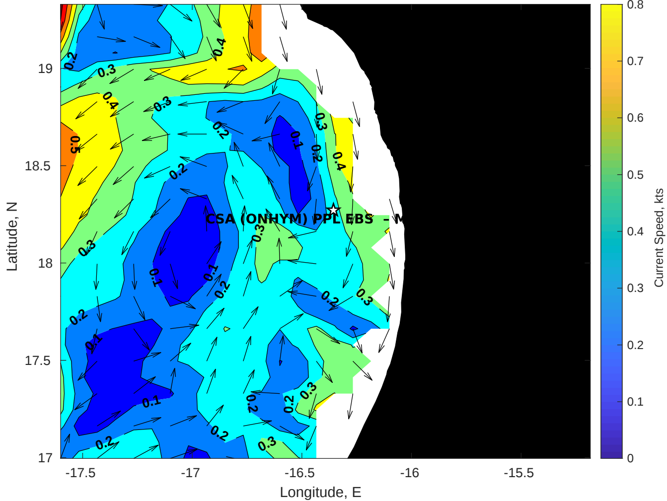
Surface Currents for CSA (ONHYM) PPL EBS - Mauritania at 18-Apr-2025 00:00:00
