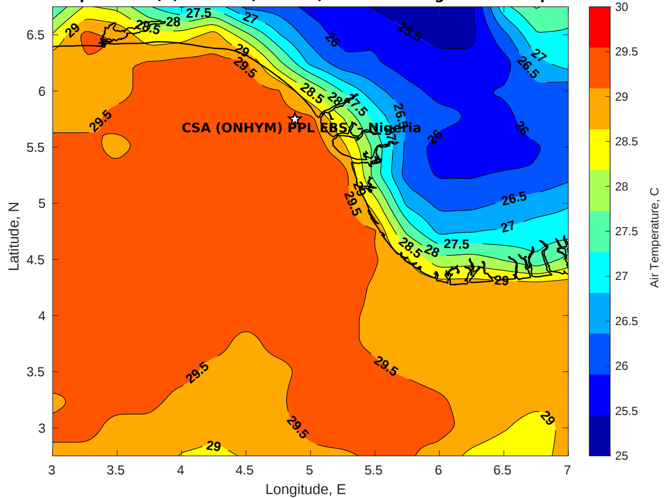
Air Temperature (C) for CSA (ONHYM) PPL EBS - Nigeria at 19-Apr-2025
