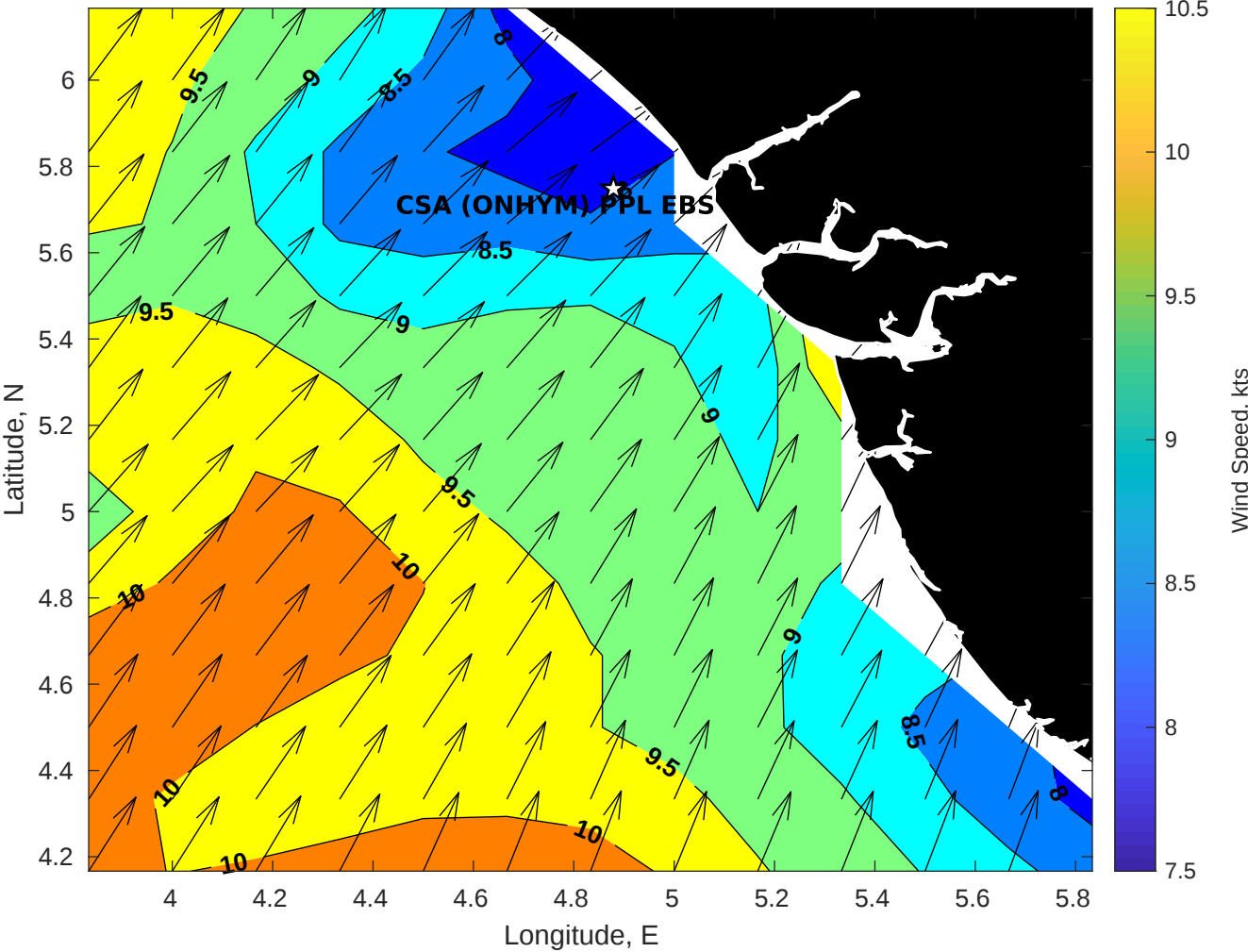
Winds (kts) for CSA (ONHYM) PPL EBS - Nigeria at 19-Apr-2025 09:00:00
