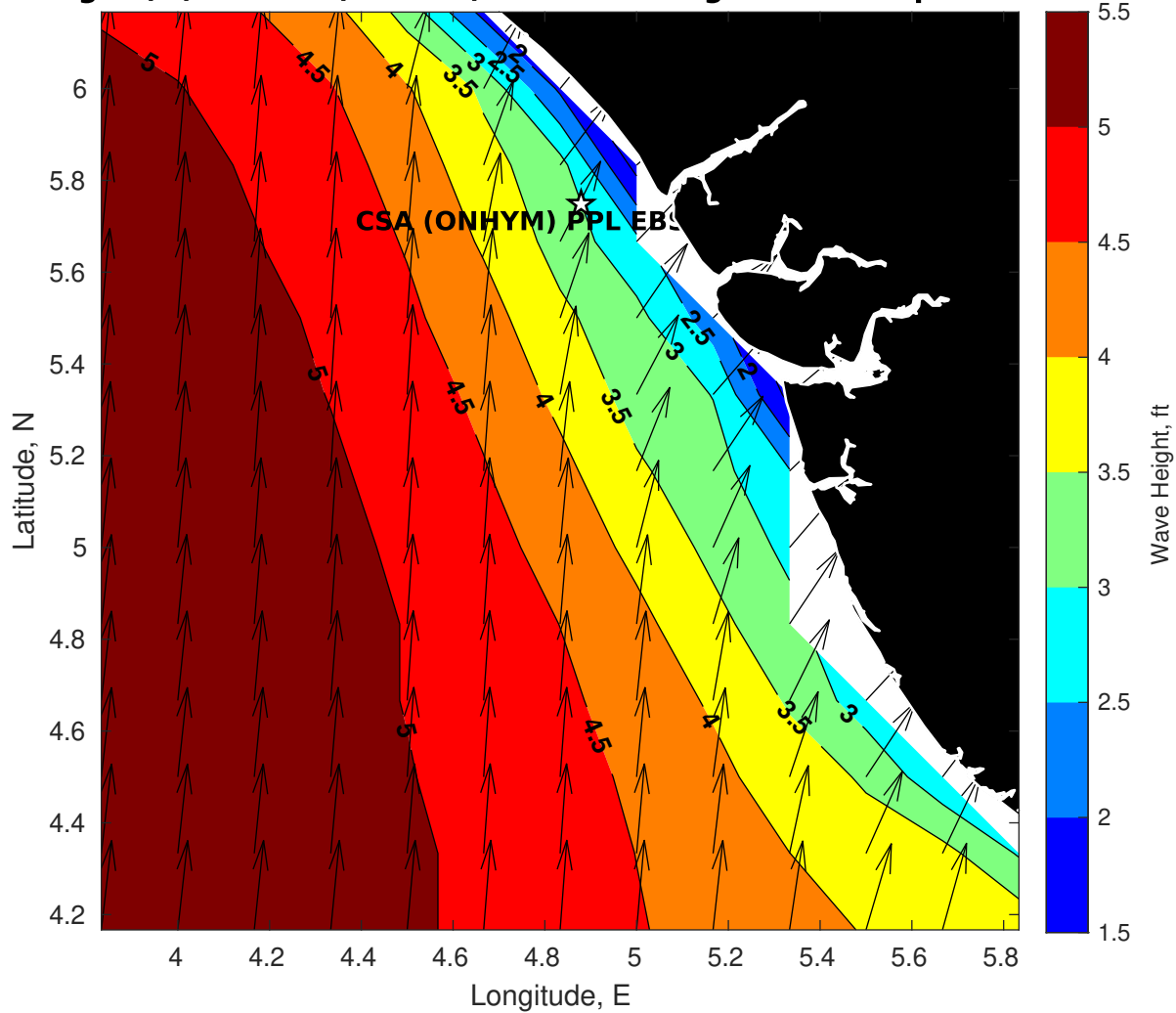
Wave Height (ft) for CSA (ONHYM) PPL EBS - Nigeria at 19-Apr-2025 09:00:00
