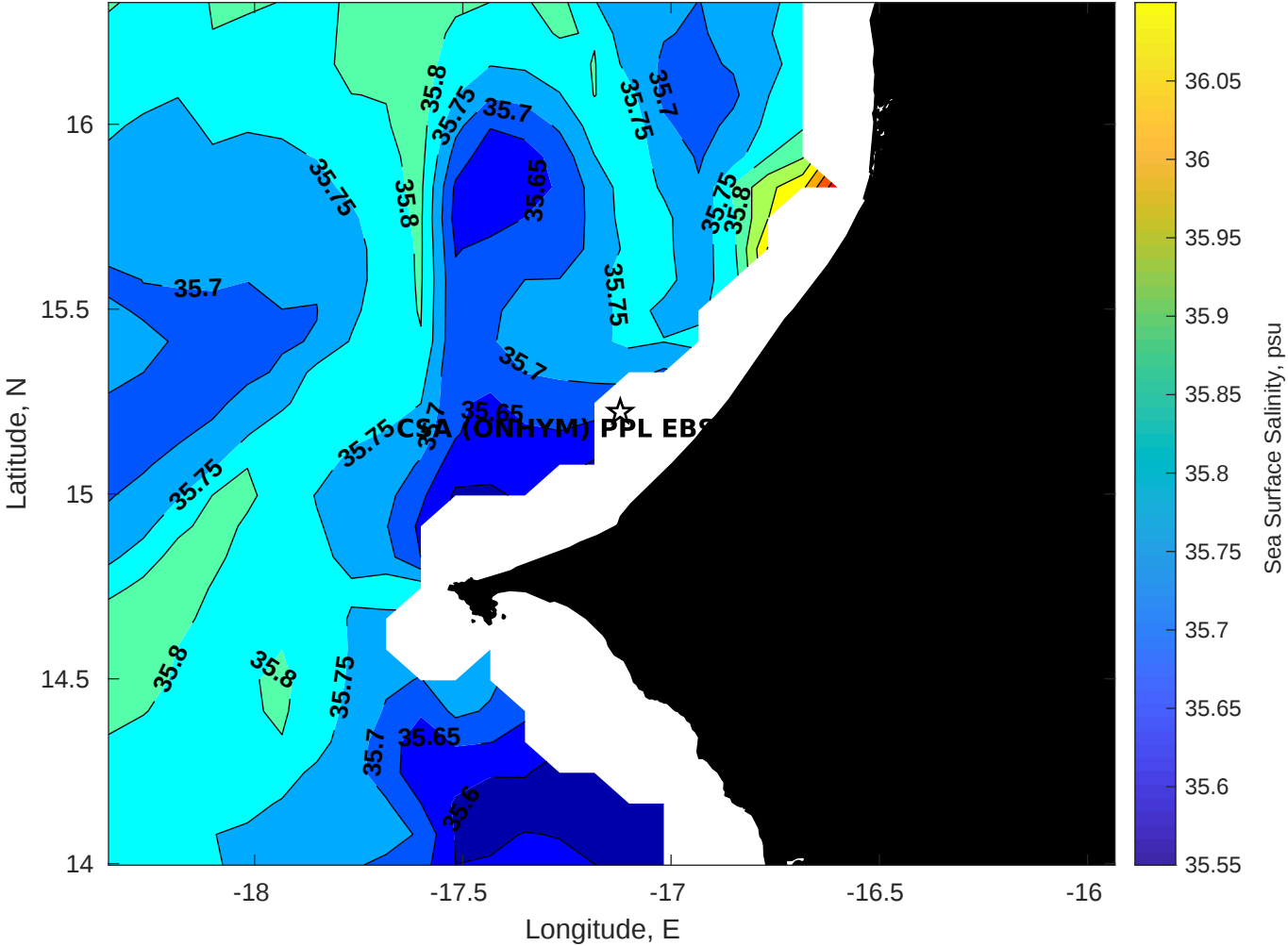
Surface Salinity for CSA (ONHYM) PPL EBS - Senegal at 18-Apr-2025 00:00:00
