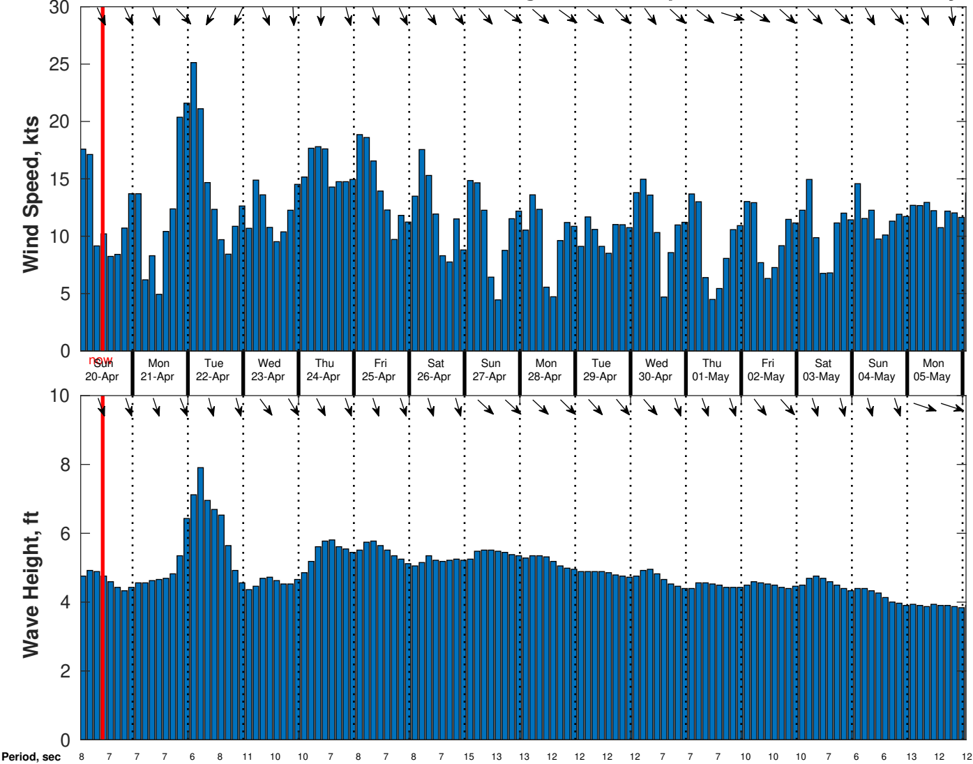
Wind & Wave Forecast for CSA (ONHYM) PPL EBS - Senegal from 19-Apr-2025 01:00:00 to 05-May-2025 01:00:00
