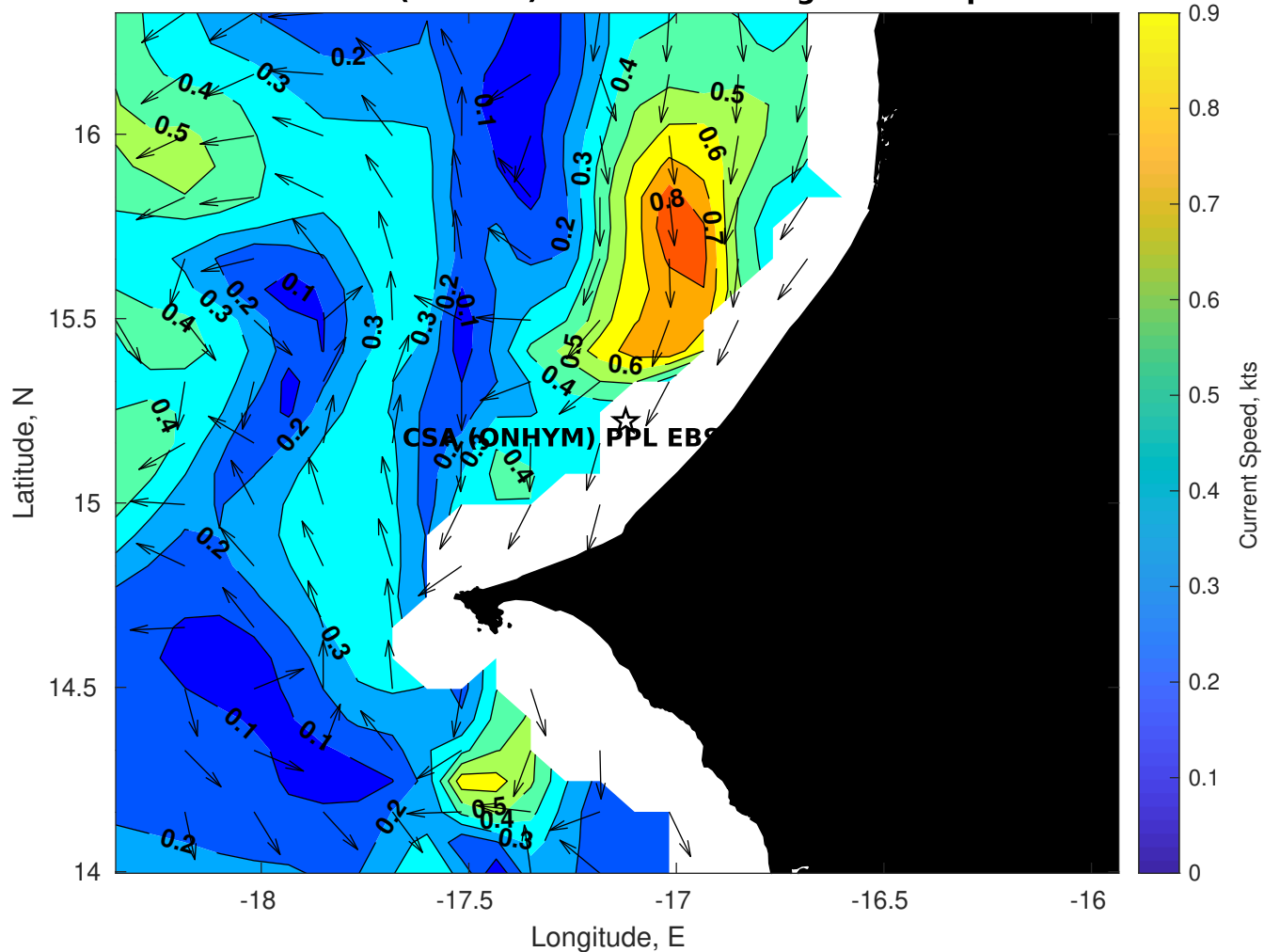
Surface Currents for CSA (ONHYM) PPL EBS - Senegal at 18-Apr-2025 00:00:00
