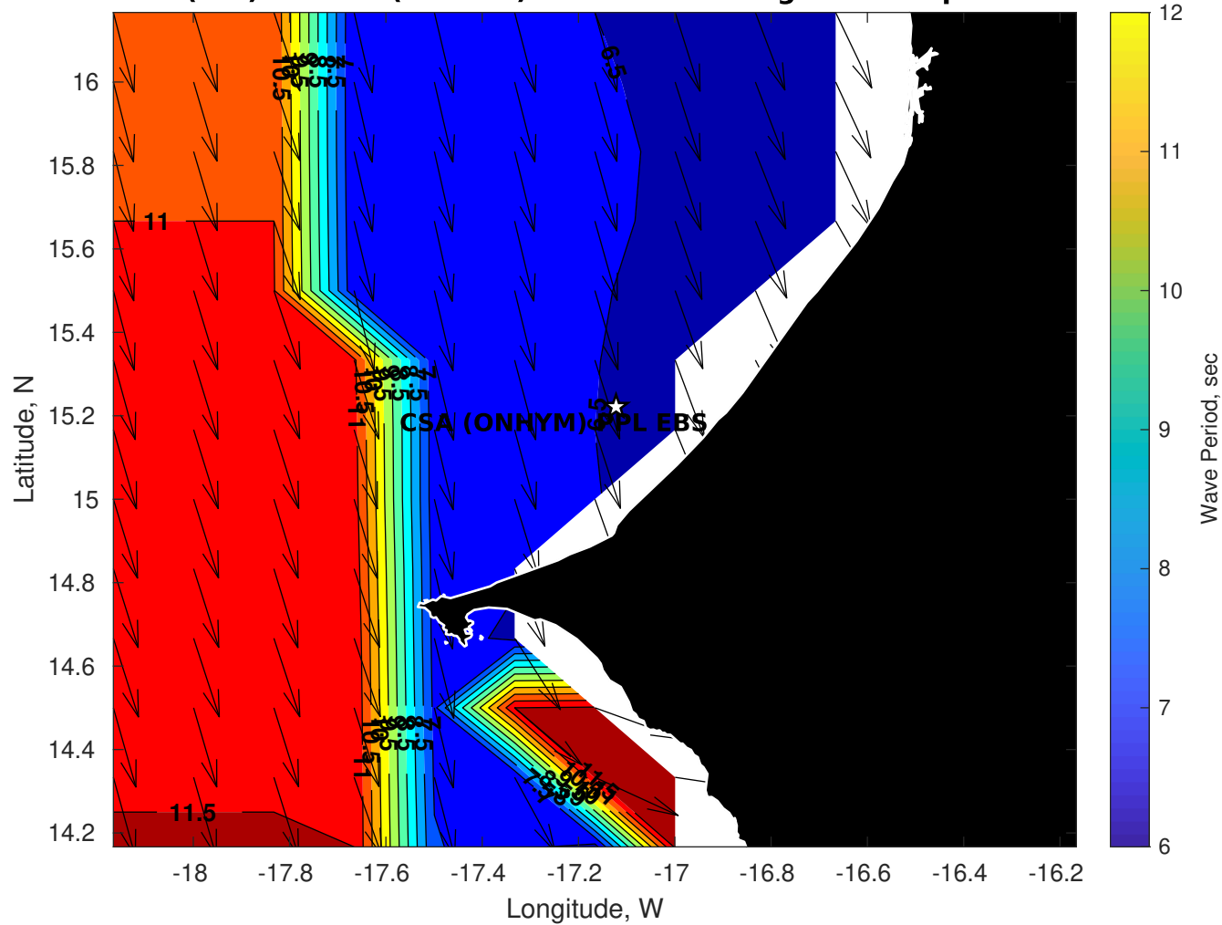
Wave Period (sec) for CSA (ONHYM) PPL EBS - Senegal at 19-Apr-2025 09:00:00
