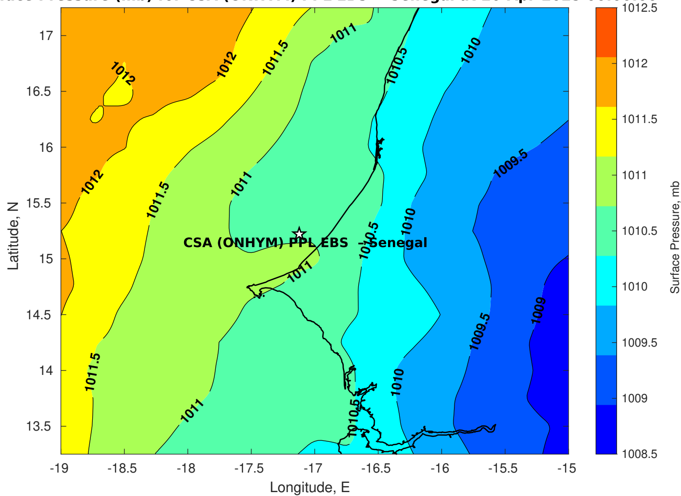
Surface Pressure (mb) for CSA (ONHYM) PPL EBS - Senegal at 20-Apr-2025 00:00:00
