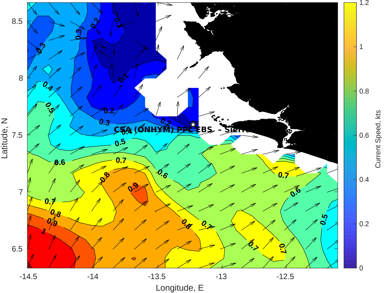
Surface Currents for CSA (ONHYM) PPL EBS - Sierra Leone at 18-Apr-2025 00:00:00
