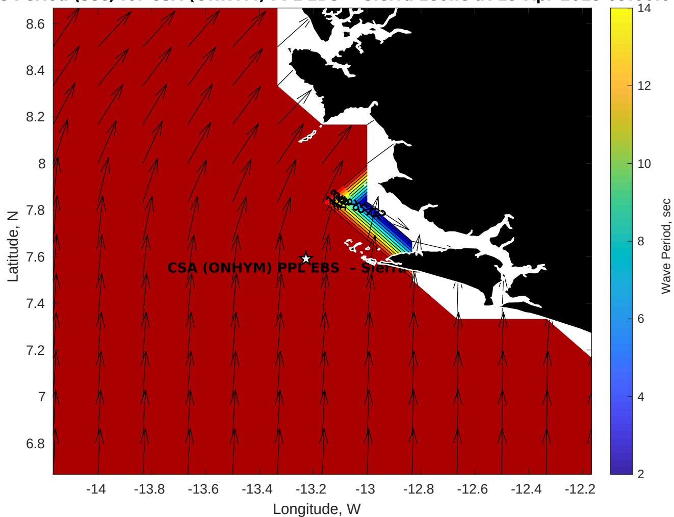
Wave Period (sec) for CSA (ONHYM) PPL EBS - Sierra Leone at 19-Apr-2025 09:00:00
