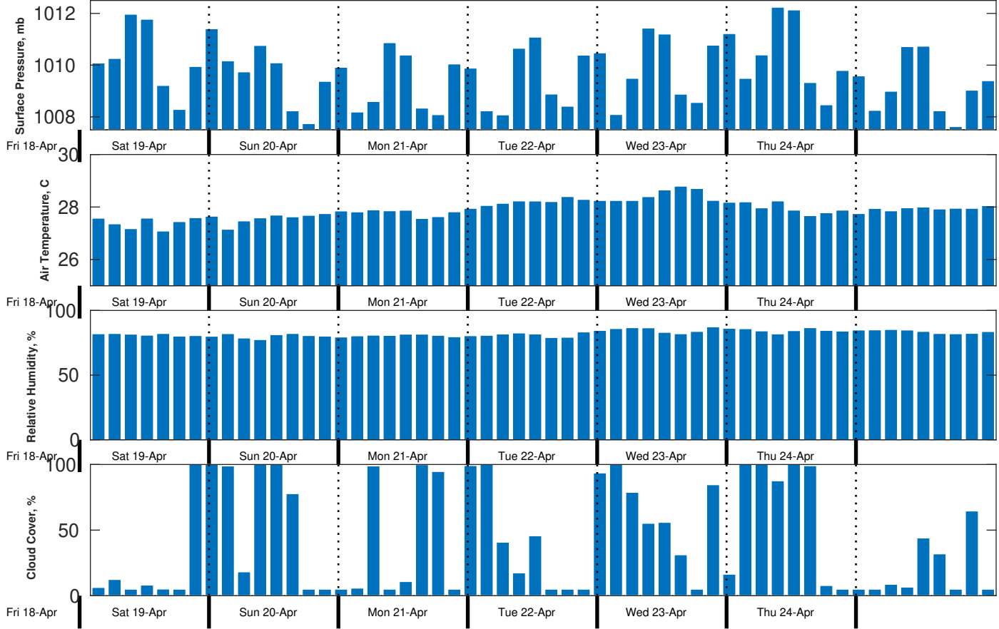
Met Forecast for CSA (ONHYM) PPL EBS - Sierra Leone from 19-Apr-2025 00:00:00 to 26-Apr-2025 00:00:00
