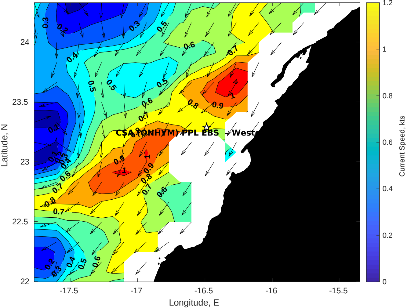
Surface Currents for CSA (ONHYM) PPL EBS - Western Sahara at 18-Apr-2025 00:00:00
