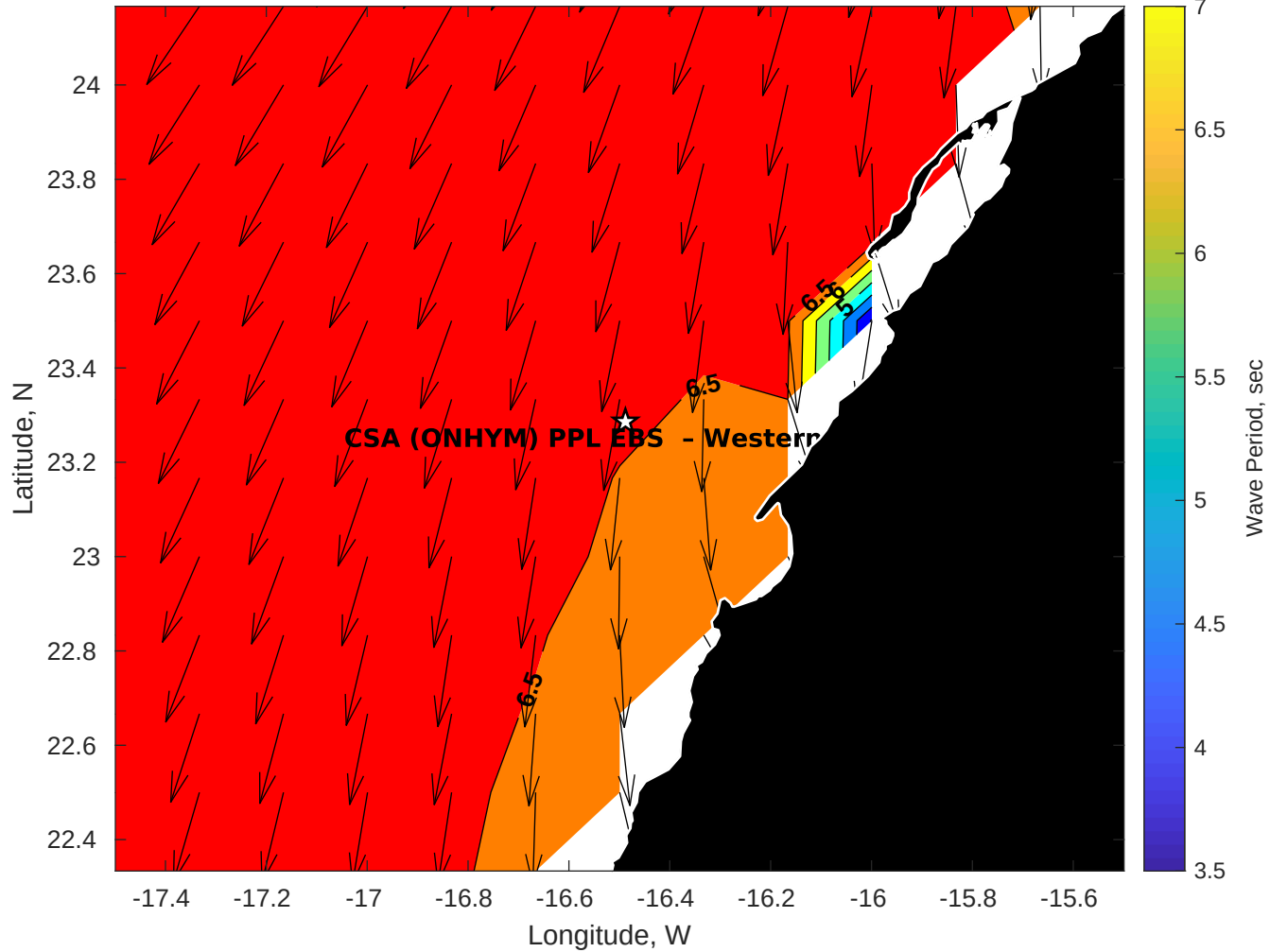
Wave Period (sec) for CSA (ONHYM) PPL EBS - Western Sahara at 19-Apr-2025 09:00:00
