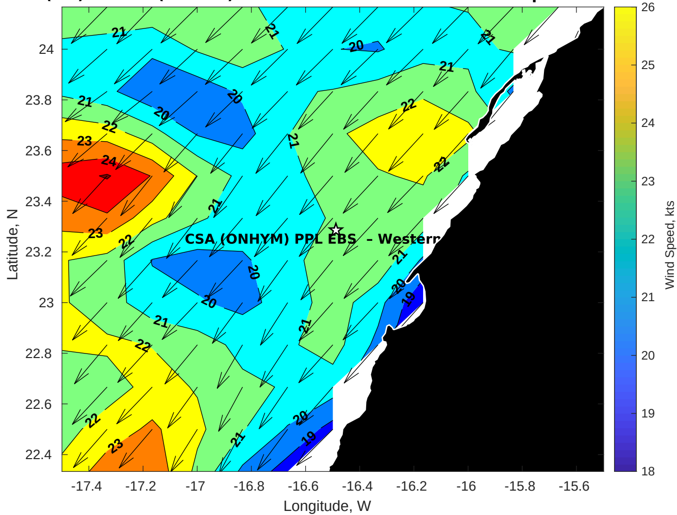
Winds (kts) for CSA (ONHYM) PPL EBS - Western Sahara at 19-Apr-2025 09:00:00
