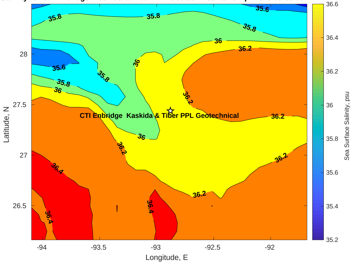
Surface Salinity for CTI Enbridge Kaskida & Tiber PPL Geotechnical at 18-Apr-2025 00:00:00
