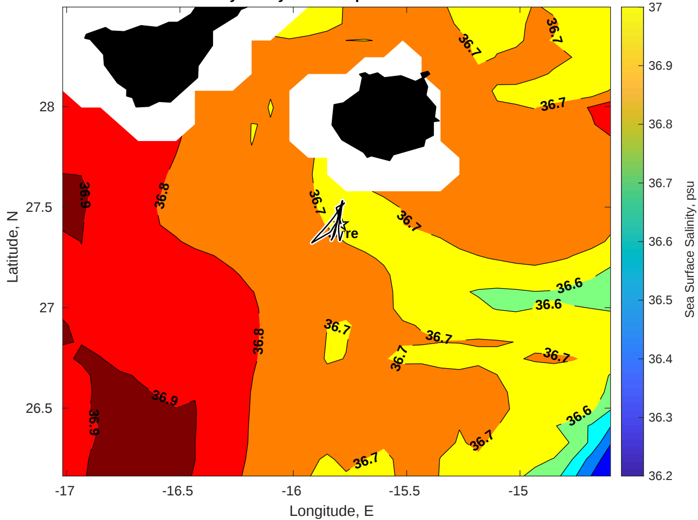
Surface Salinity for Gyre at 18-Apr-2025 00:00:00
