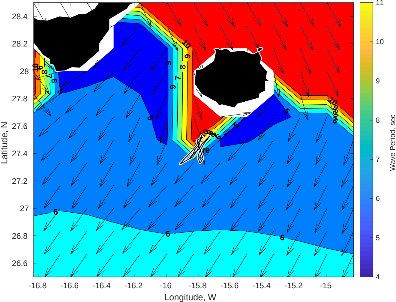
Wave Period (sec) for Gyre at 19-Apr-2025 09:00:00
