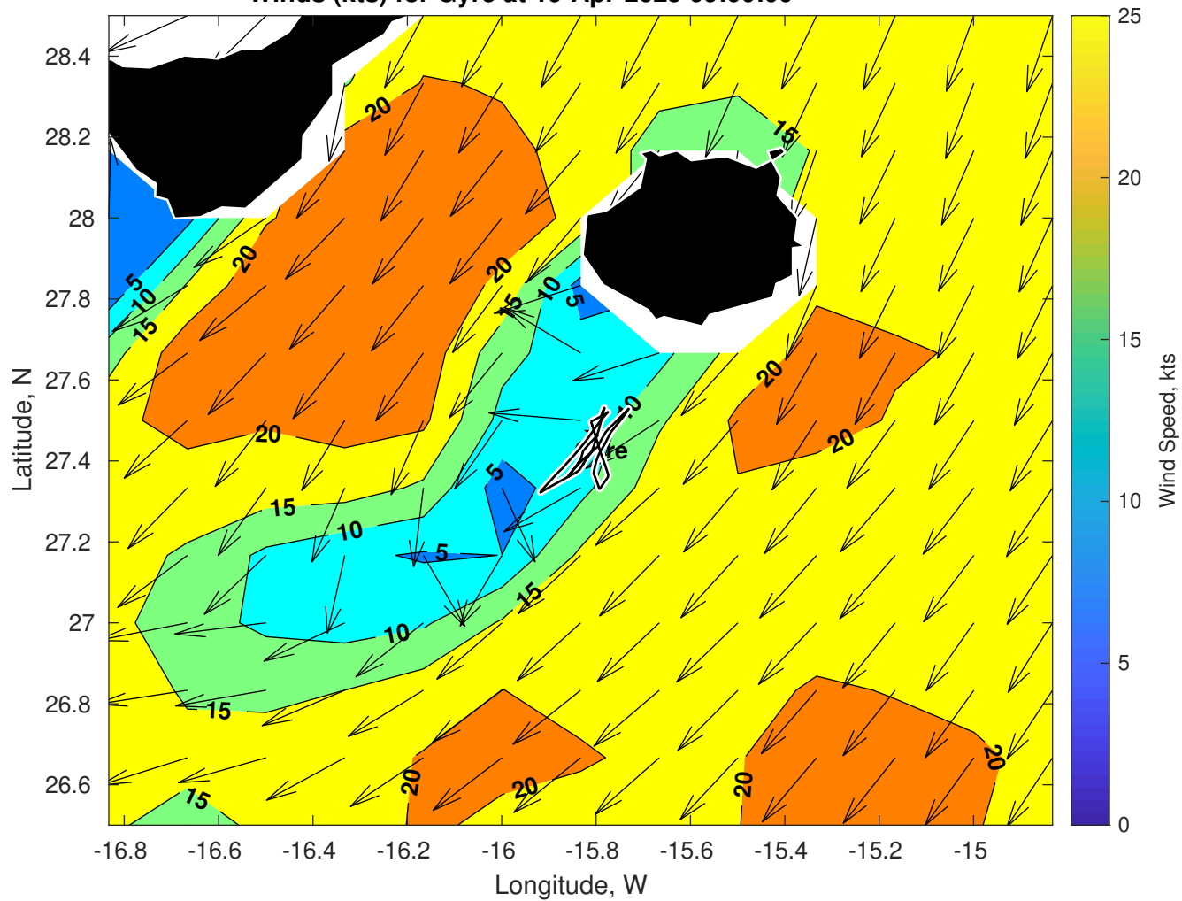
Winds (kts) for Gyre at 19-Apr-2025 09:00:00
