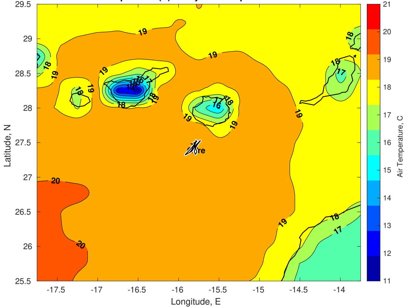
Air Temperature (C) for Gyre at 19-Apr-2025
