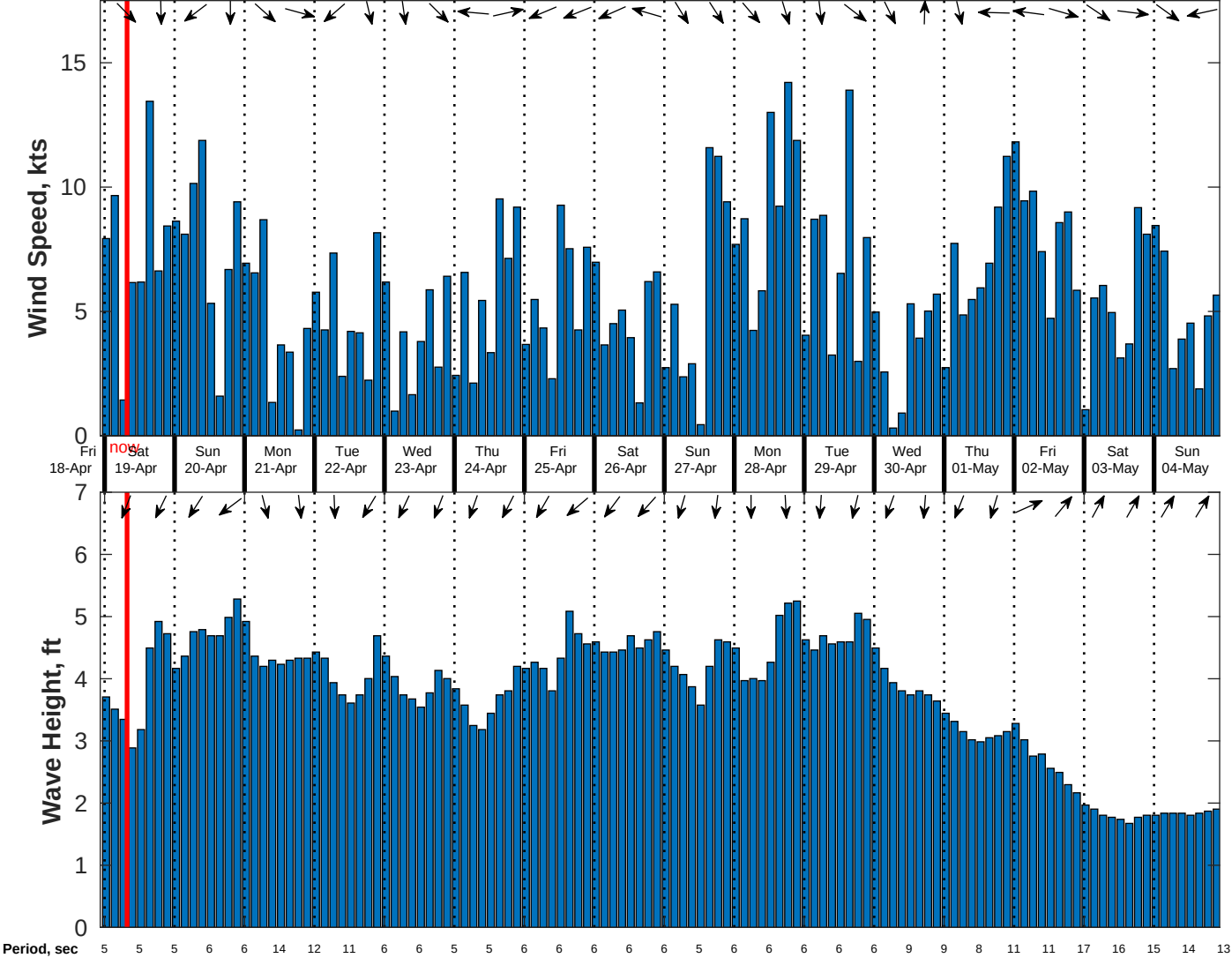
Wind & Wave Forecast for Gyre from 18-Apr-2025 23:00:00 to 04-May-2025 23:00:00
