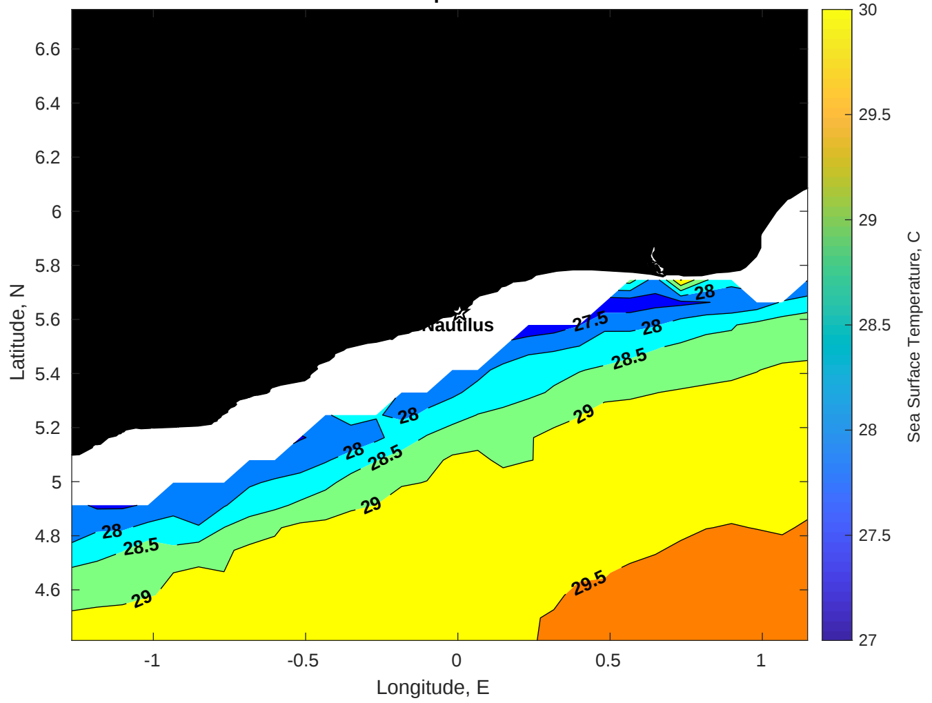
SST for Nautilus at 18-Apr-2025 00:00:00
