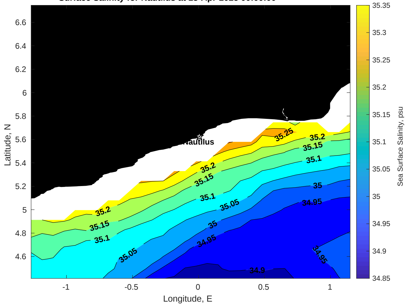
Surface Salinity for Nautilus at 18-Apr-2025 00:00:00
