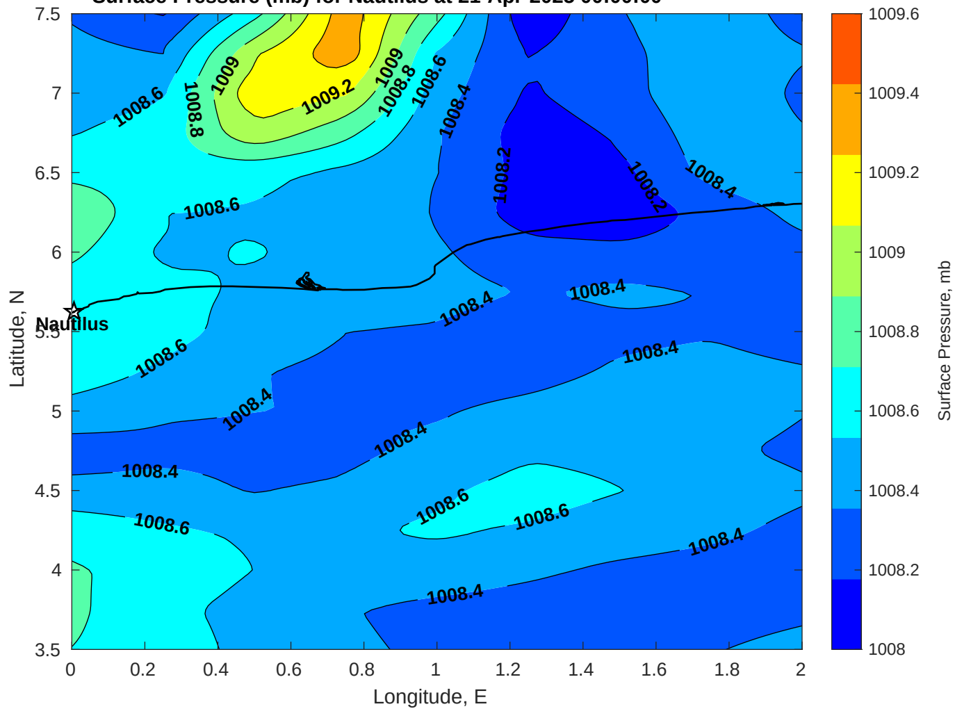
Surface Pressure (mb) for Nautilus at 21-Apr-2025 00:00:00
