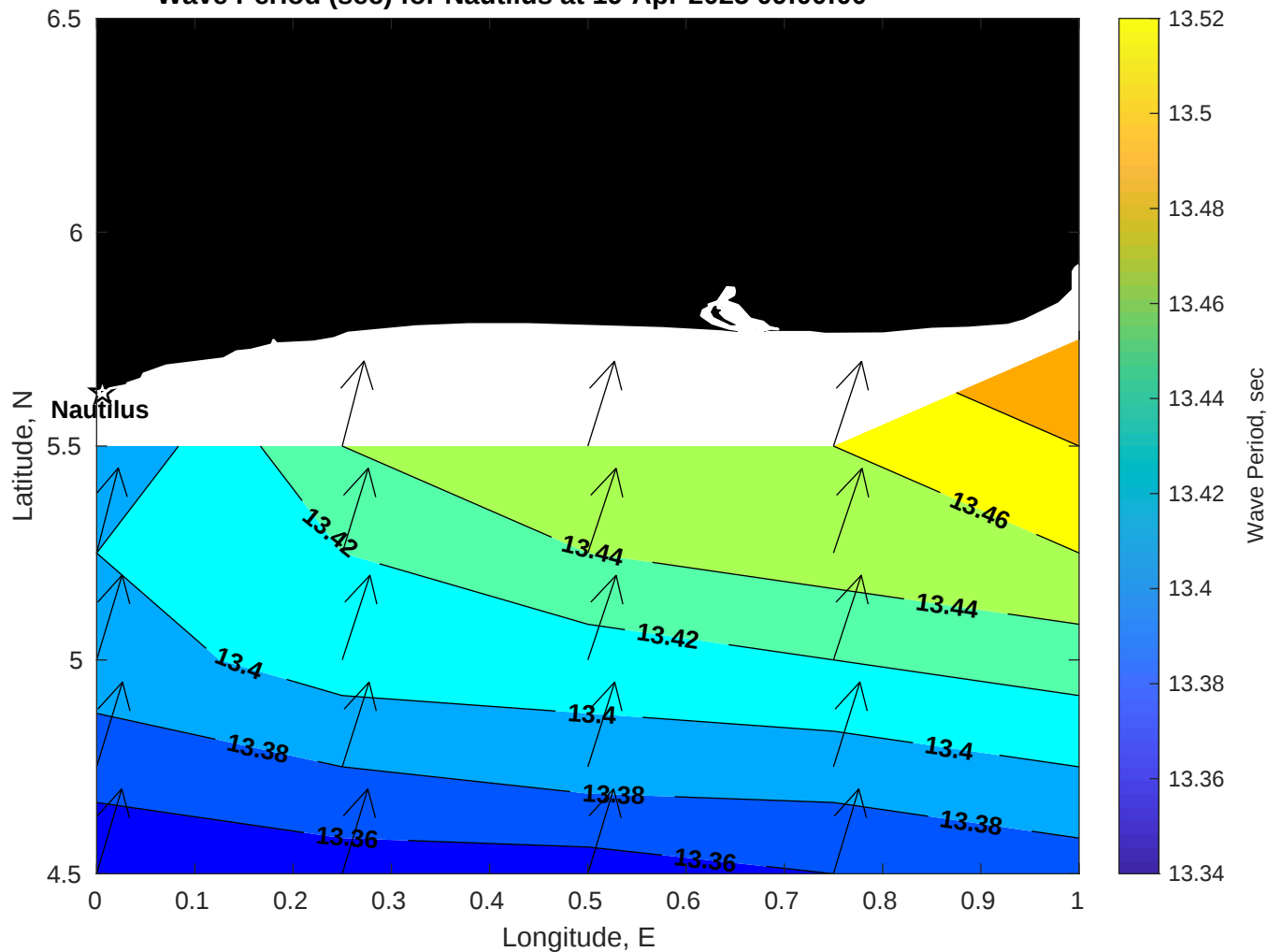
Wave Period (sec) for Nautilus at 19-Apr-2025 09:00:00
