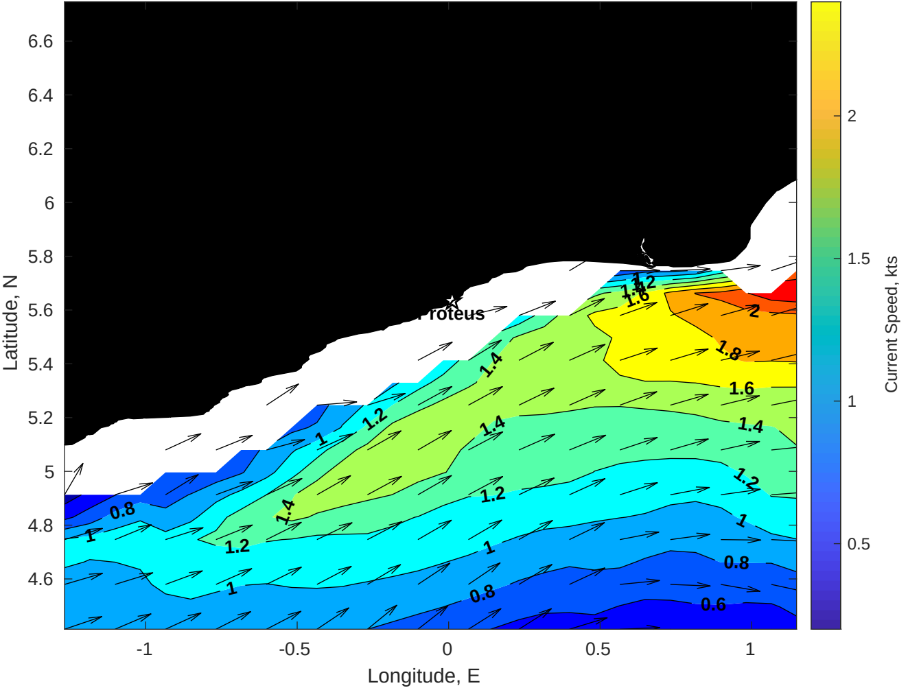
Surface Currents for Proteus at 18-Apr-2025 00:00:00
