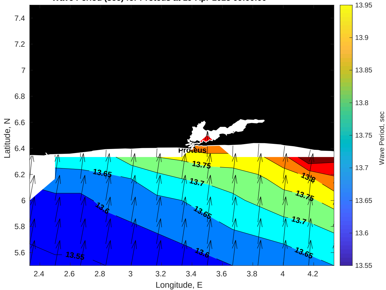
Wave Period (sec) for Proteus at 19-Apr-2025 09:00:00
