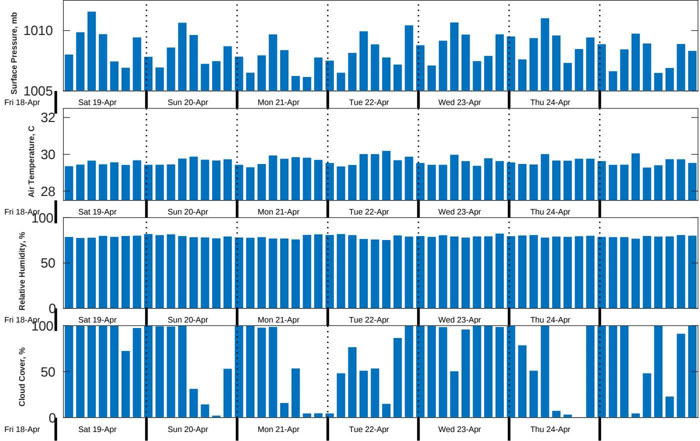
Met Forecast for Proteus from 19-Apr-2025 00:00:00 to 26-Apr-2025 00:00:00
