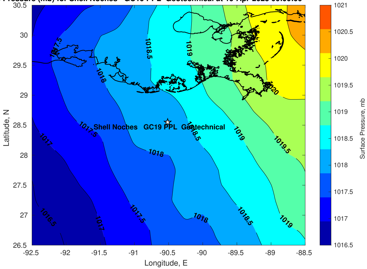
Surface Pressure (mb) for Shell Noches GC19 PPL Geotechnical at 19-Apr-2025 00:00:00
