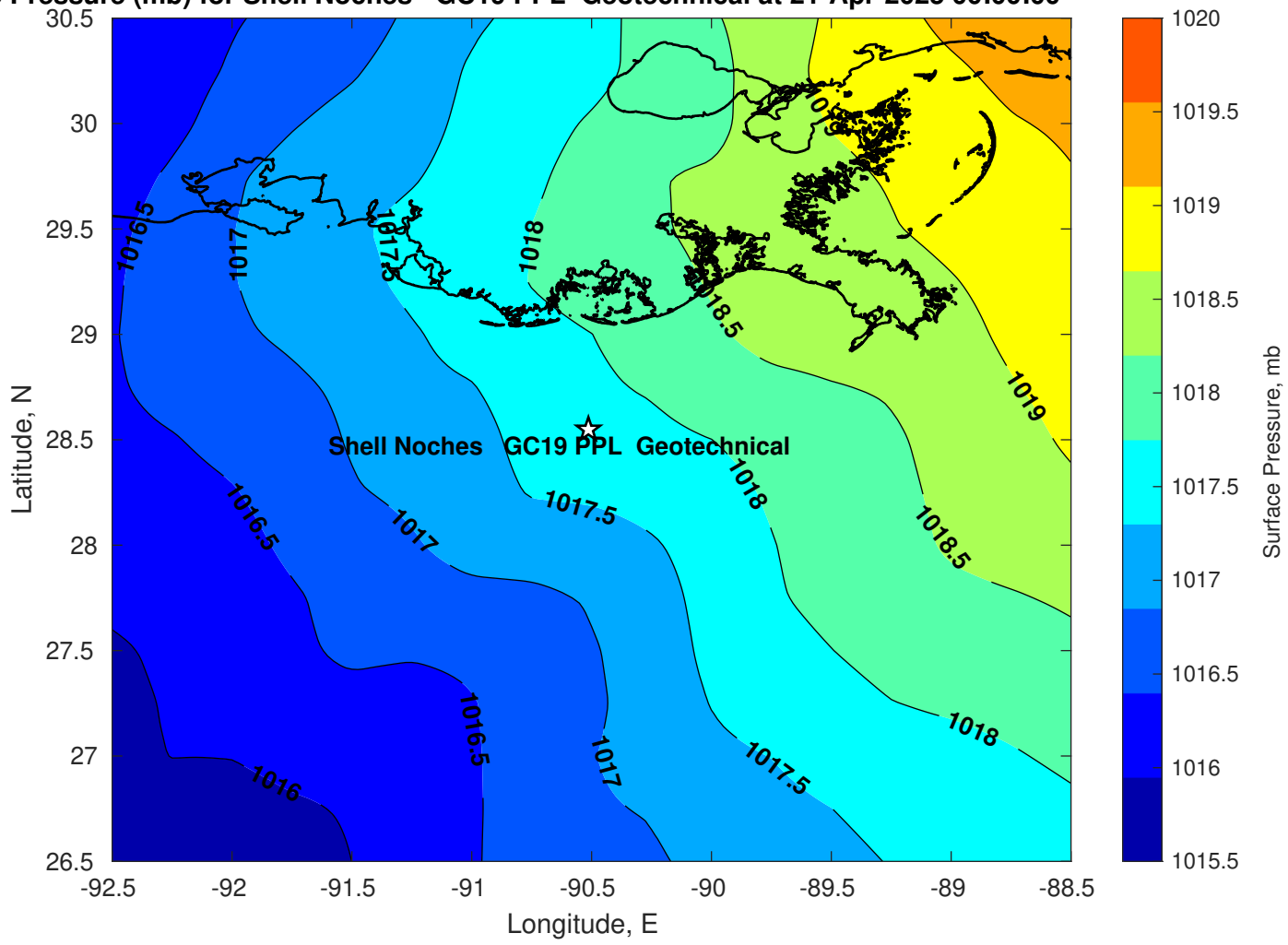
Surface Pressure (mb) for Shell Noches GC19 PPL Geotechnical at 21-Apr-2025 00:00:00
