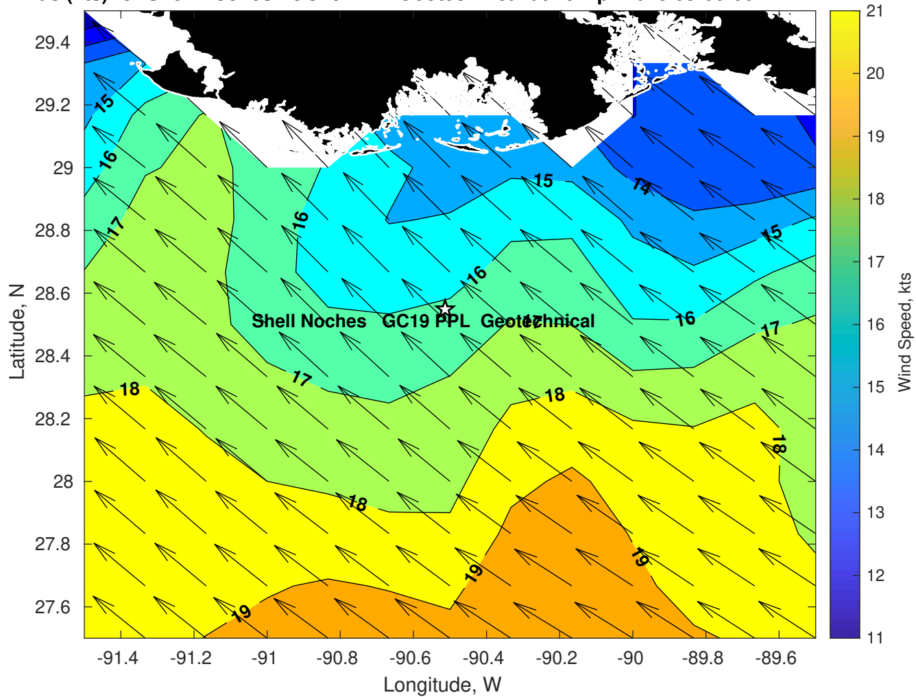
Winds (kts) for Shell Noches GC19 PPL Geotechnical at 19-Apr-2025 09:00:00
