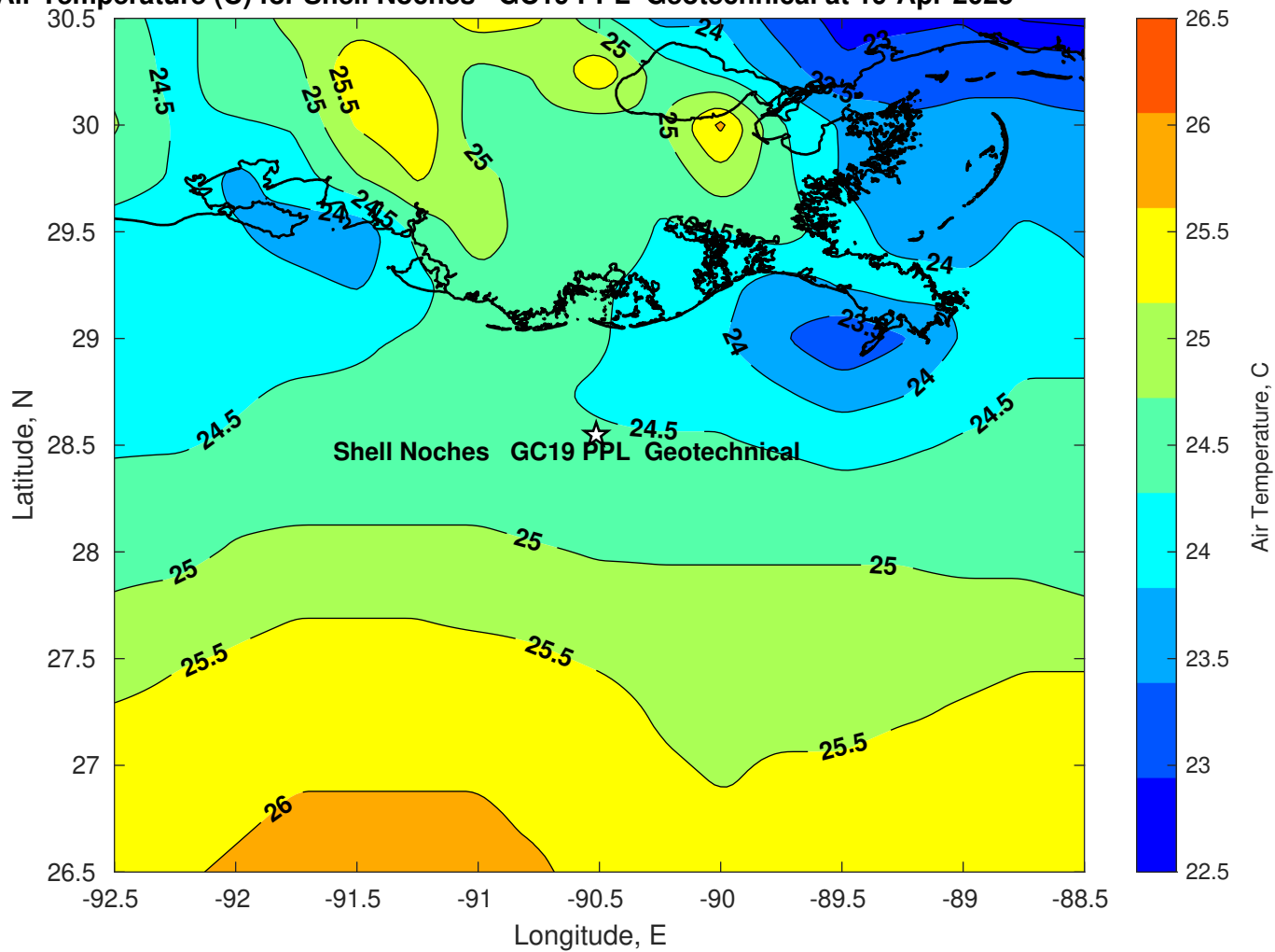
Air Temperature (C) for Shell Noches GC19 PPL Geotechnical at 19-Apr-2025
