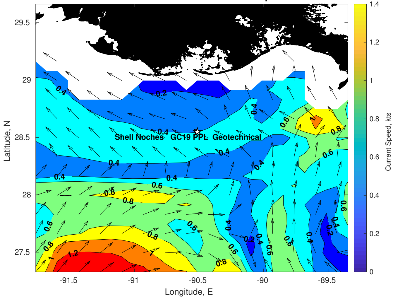
Surface Currents for Shell Noches GC19 PPL Geotechnical at 18-Apr-2025 00:00:00
