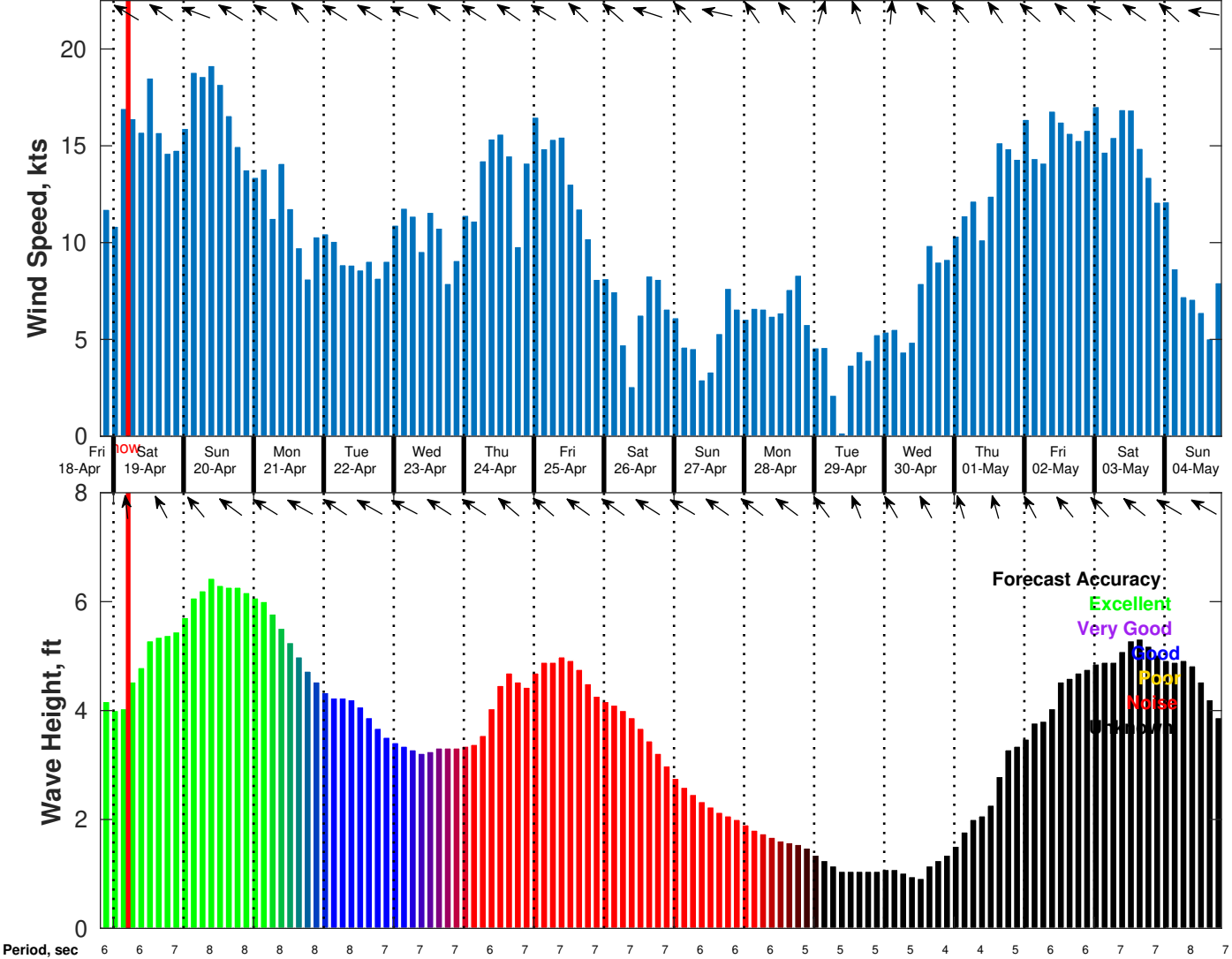
Wind & Wave Forecast for Shell Noches GC19 PPL Geotechnical from 18-Apr-2025 20:00:00 to 04-May-2025 20:00:00
