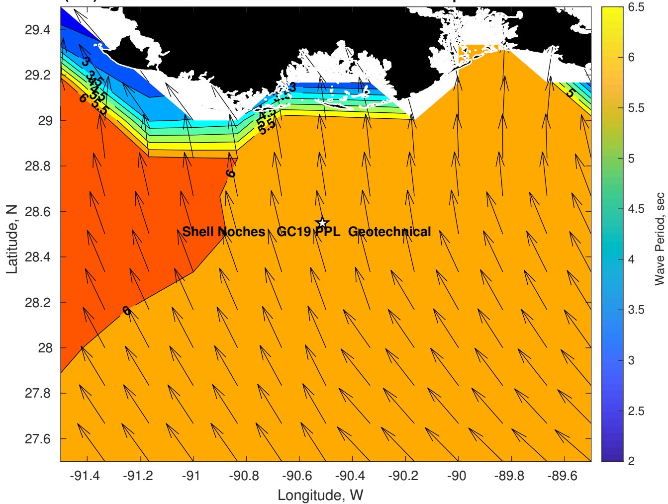
Wave Period (sec) for Shell Noches GC19 PPL Geotechnical at 19-Apr-2025 09:00:00
