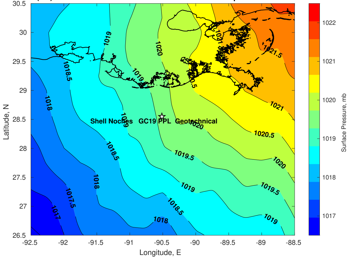
Surface Pressure (mb) for Shell Noches GC19 PPL Geotechnical at 20-Apr-2025 00:00:00
