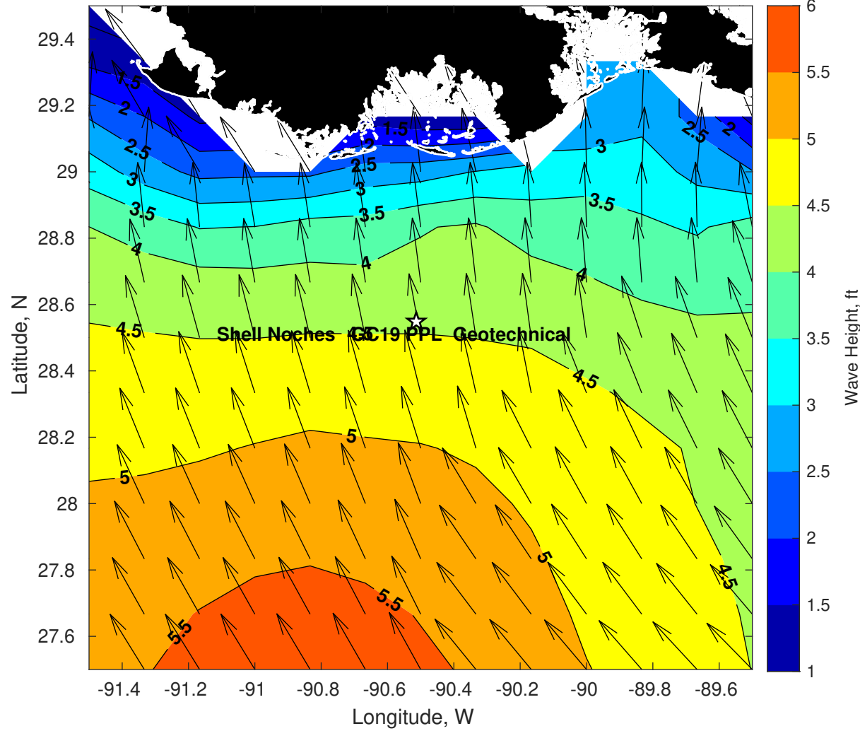
Wave Height (ft) for Shell Noches GC19 PPL Geotechnical at 19-Apr-2025 09:00:00
