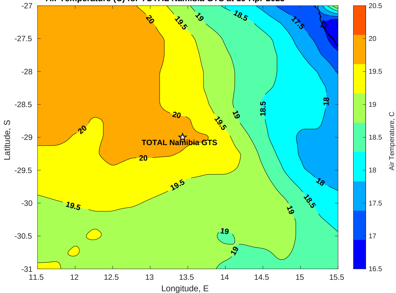
Air Temperature (C) for TOTAL Namibia GTS at 19-Apr-2025
