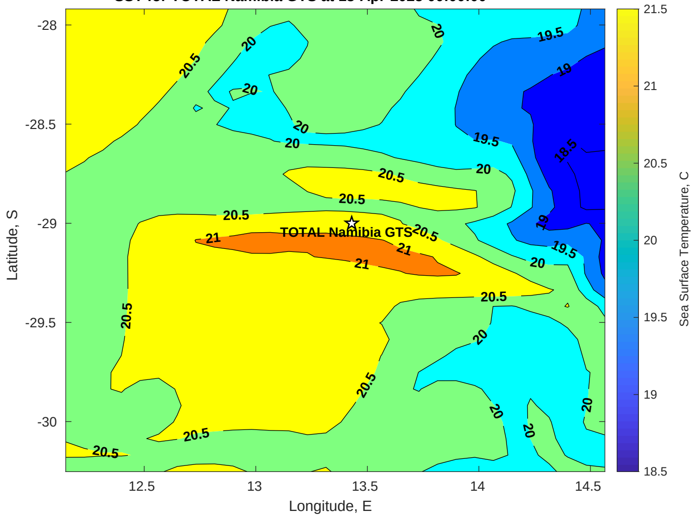
SST for TOTAL Namibia GTS at 18-Apr-2025 00:00:00
