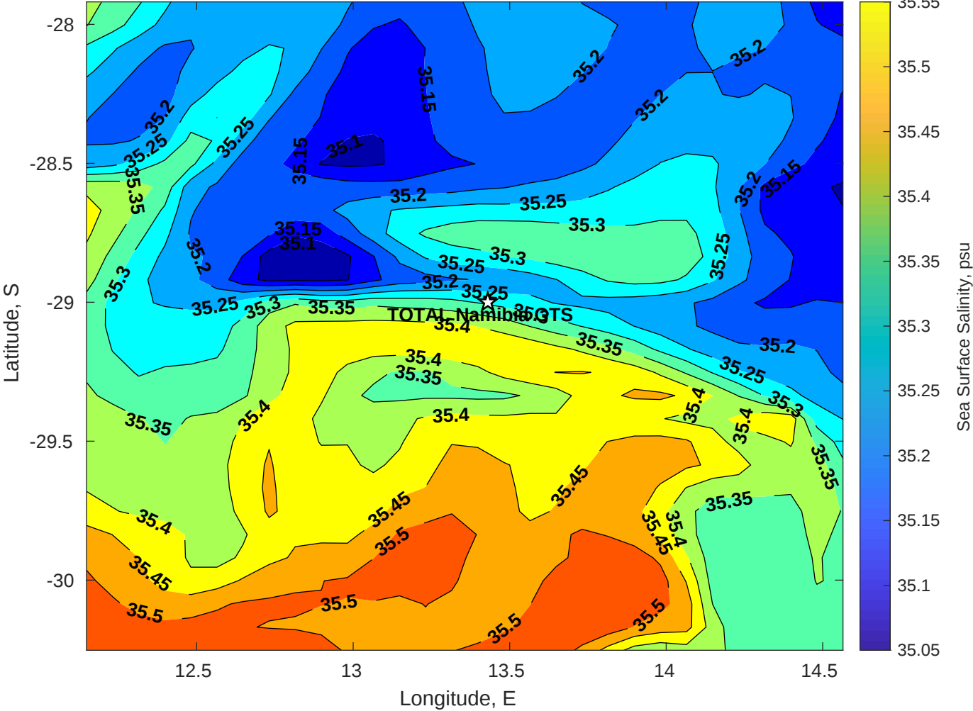
Surface Salinity for TOTAL Namibia GTS at 18-Apr-2025 00:00:00
