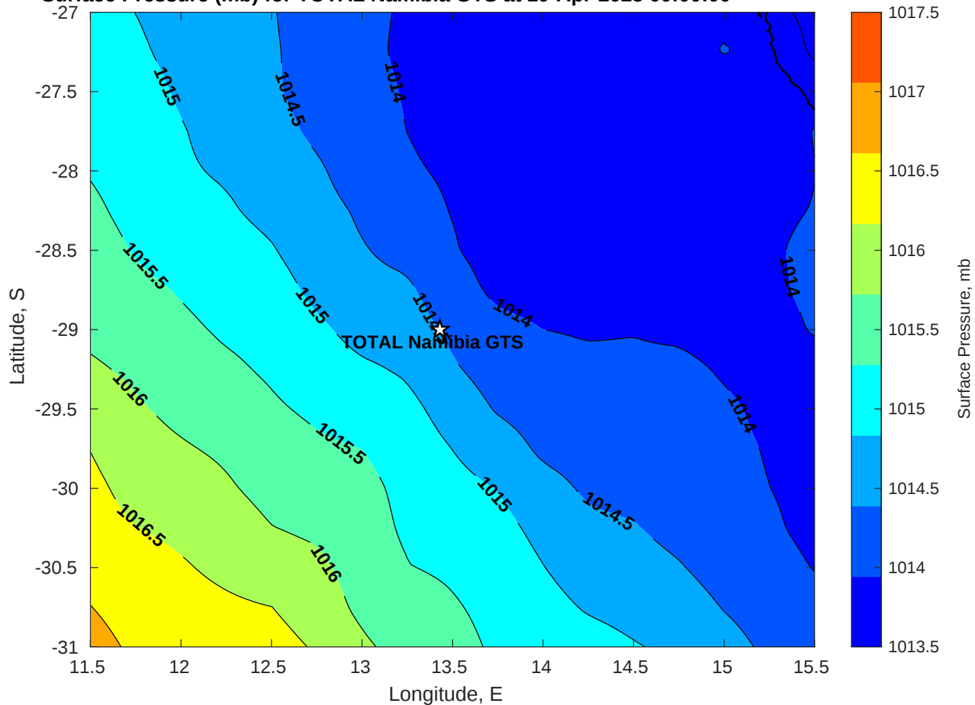
Surface Pressure (mb) for TOTAL Namibia GTS at 19-Apr-2025 00:00:00
