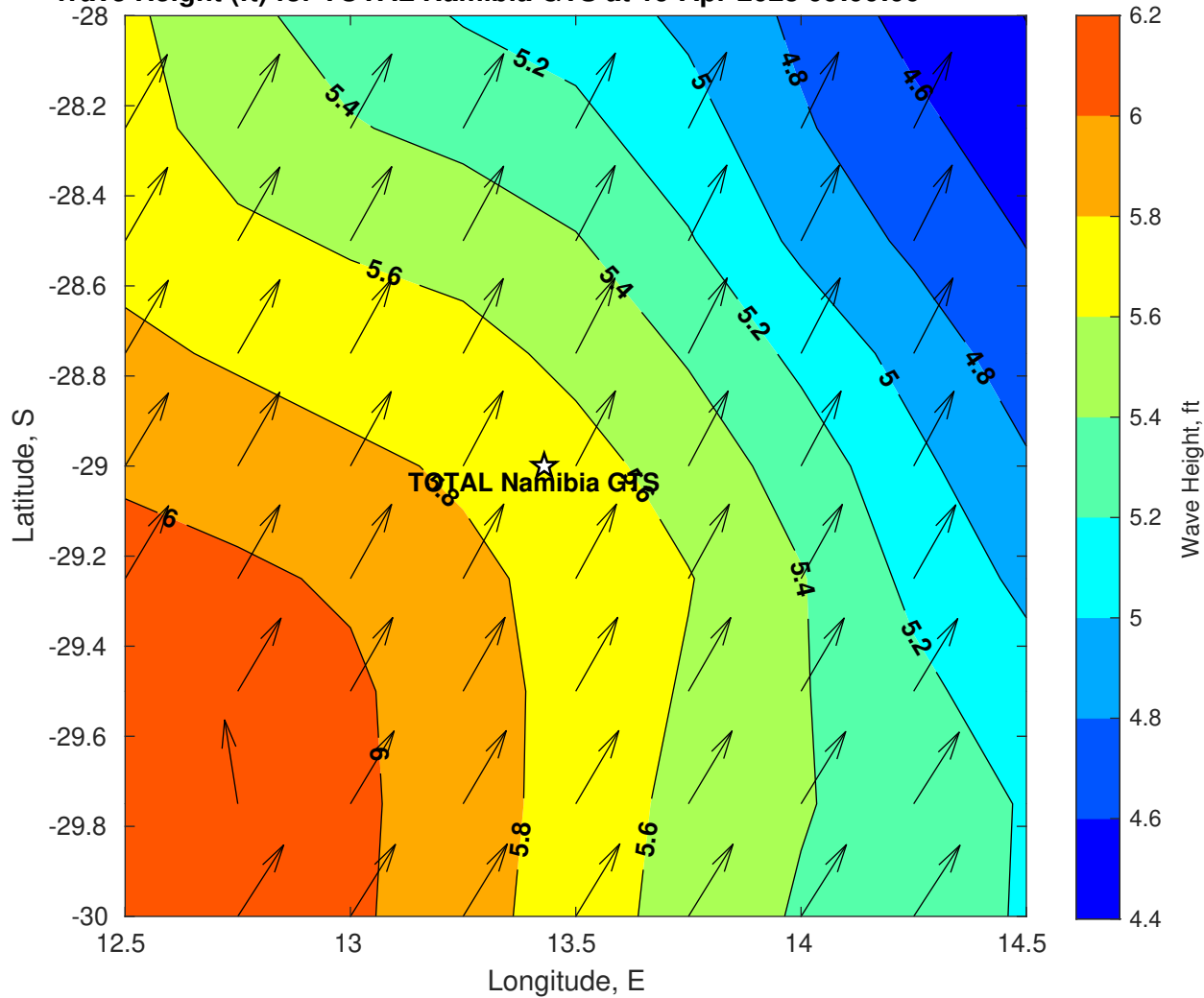
Wave Height (ft) for TOTAL Namibia GTS at 19-Apr-2025 09:00:00
