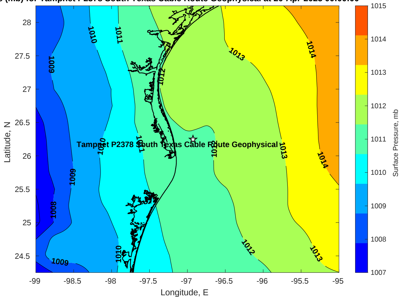
Pressure (mb) for Tampnet P2378 South Texas Cable Route Geophysical at 20-Apr-2025 00:00:00
