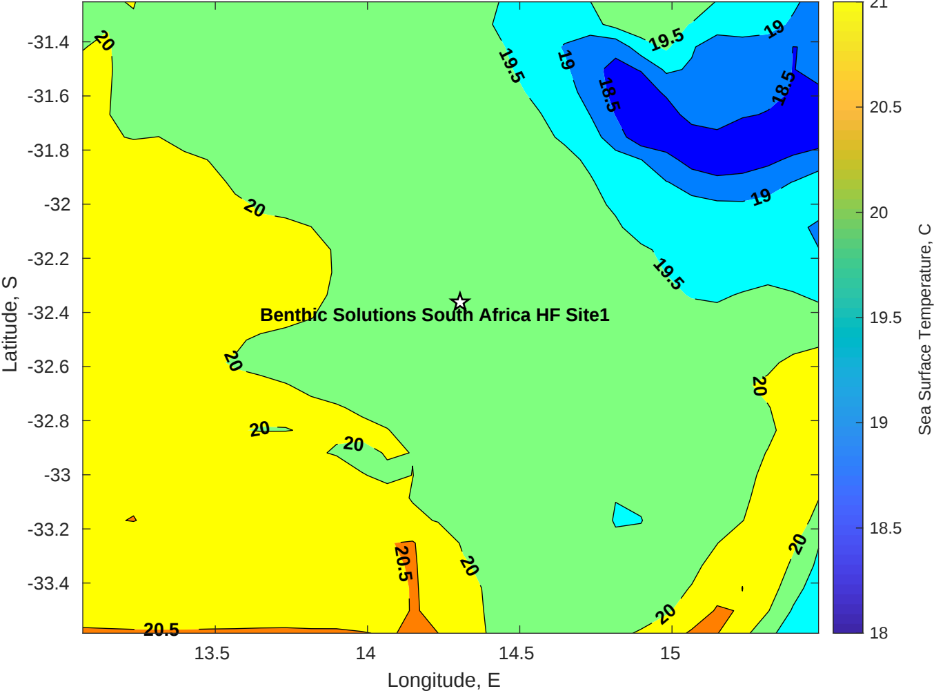
SST for Benthic Solutions South Africa HF Site1 at 19-Apr-2025 00:00:00
