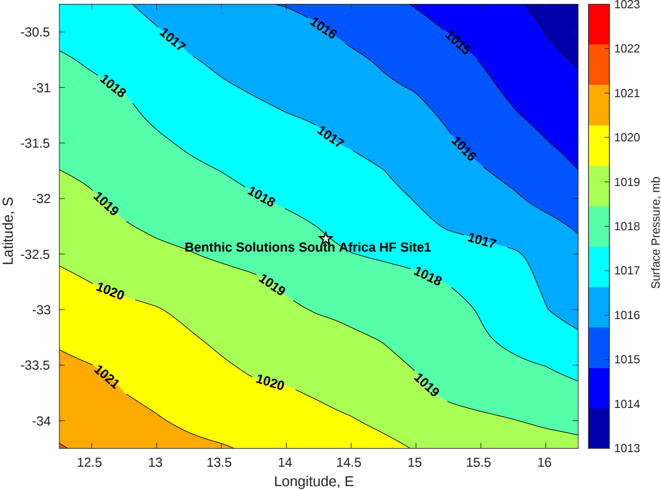
Surface Pressure (mb) for Benthic Solutions South Africa HF Site1 at 21-Apr-2025 00:00:00
