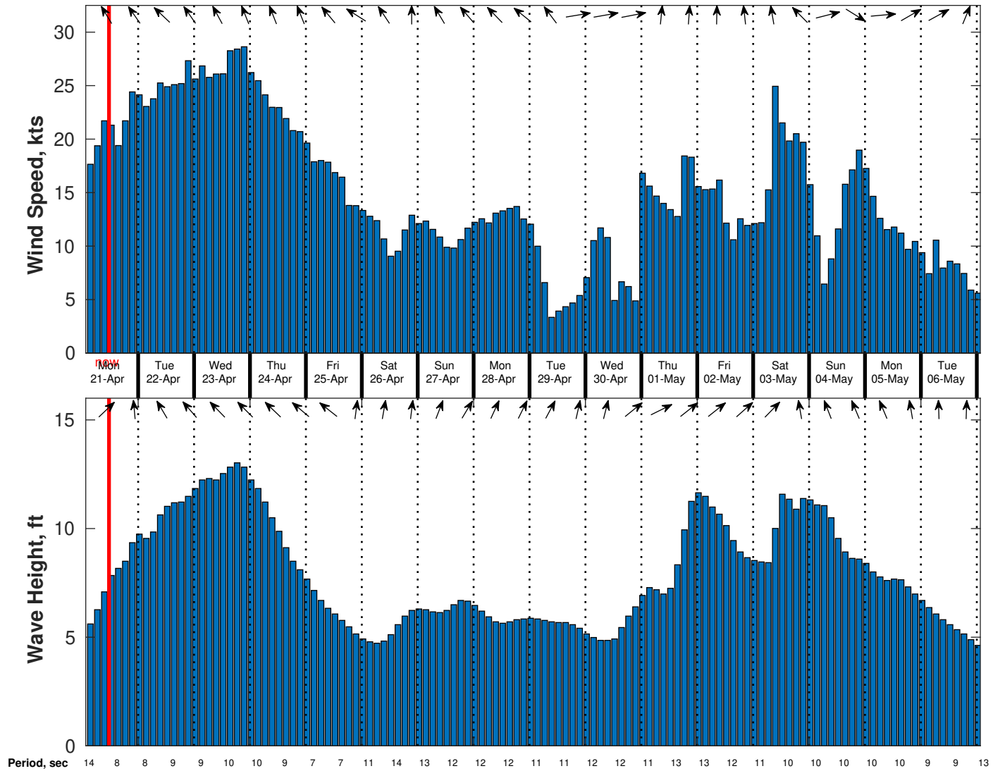
Wind & Wave Forecast for Benthic Solutions South Africa HF Site1 from 20-Apr-2025 02:00:00 to 06-May-2025 02:00:00
