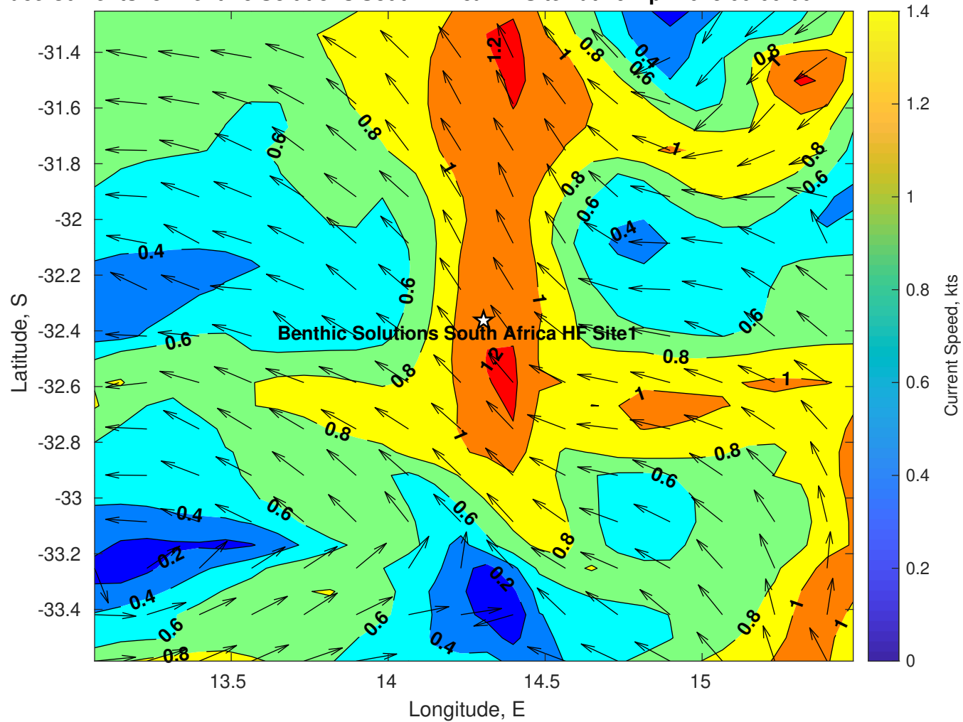
Surface Currents for Benthic Solutions South Africa HF Site1 at 19-Apr-2025 00:00:00
