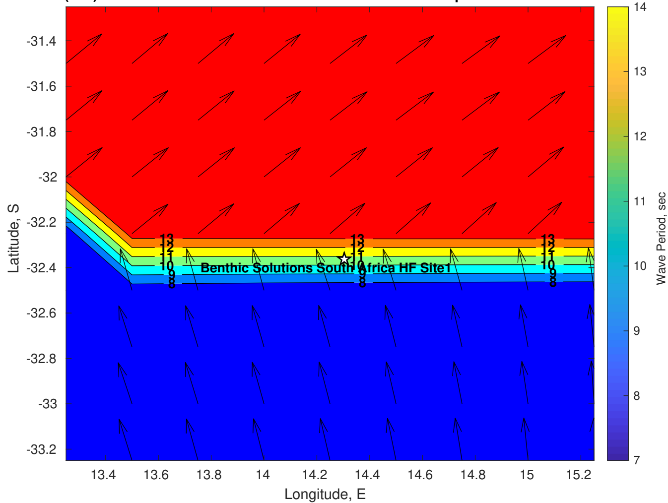
Wave Period (sec) for Benthic Solutions South Africa HF Site1 at 20-Apr-2025 09:00:00
