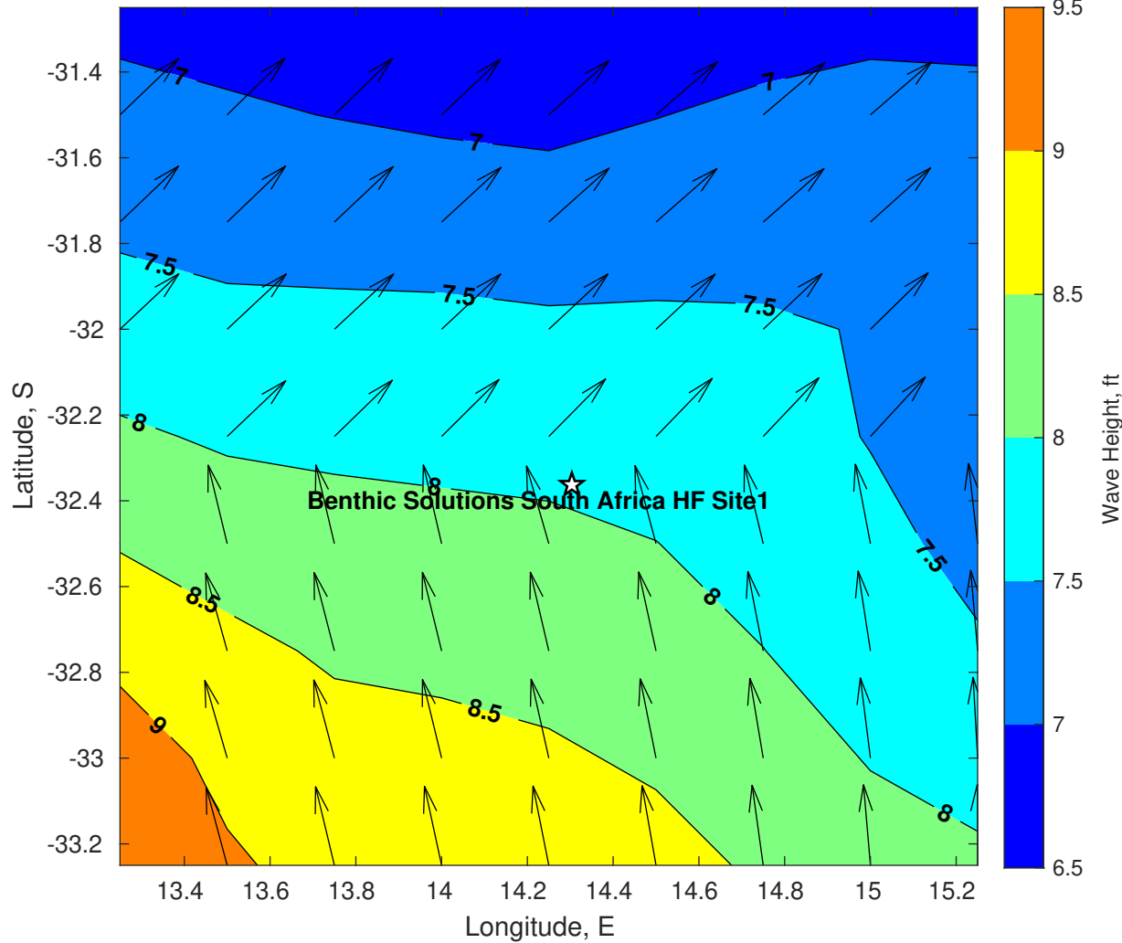
Wave Height (ft) for Benthic Solutions South Africa HF Site1 at 20-Apr-2025 09:00:00
