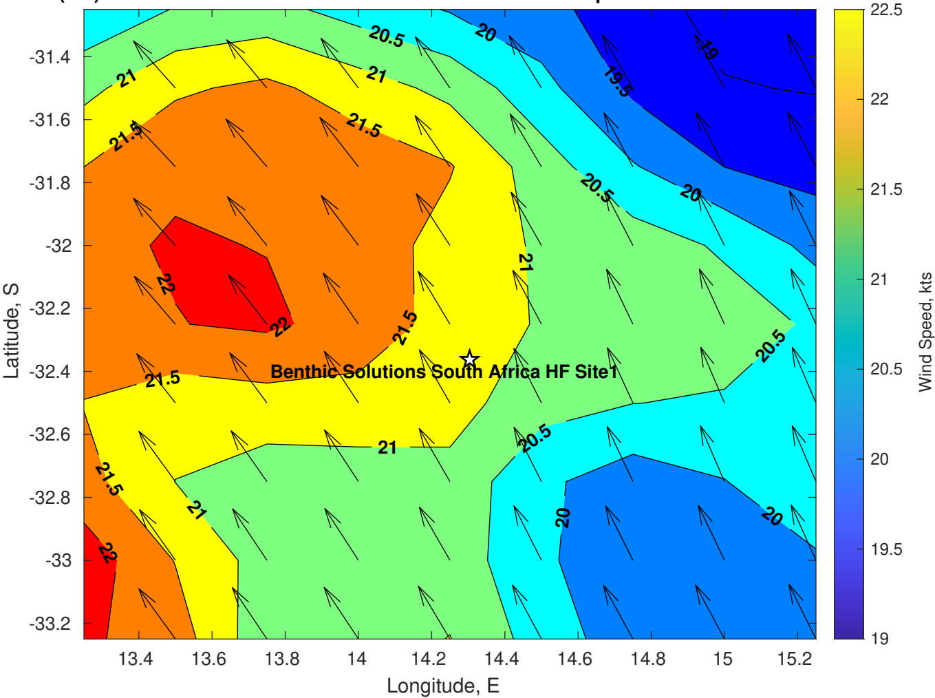
Winds (kts) for Benthic Solutions South Africa HF Site1 at 20-Apr-2025 09:00:00
