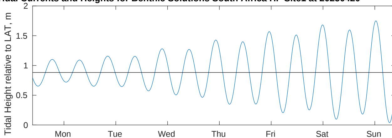
Tidal Currents and Heights for Benthic Solutions South Africa HF Site1 at 20250420
