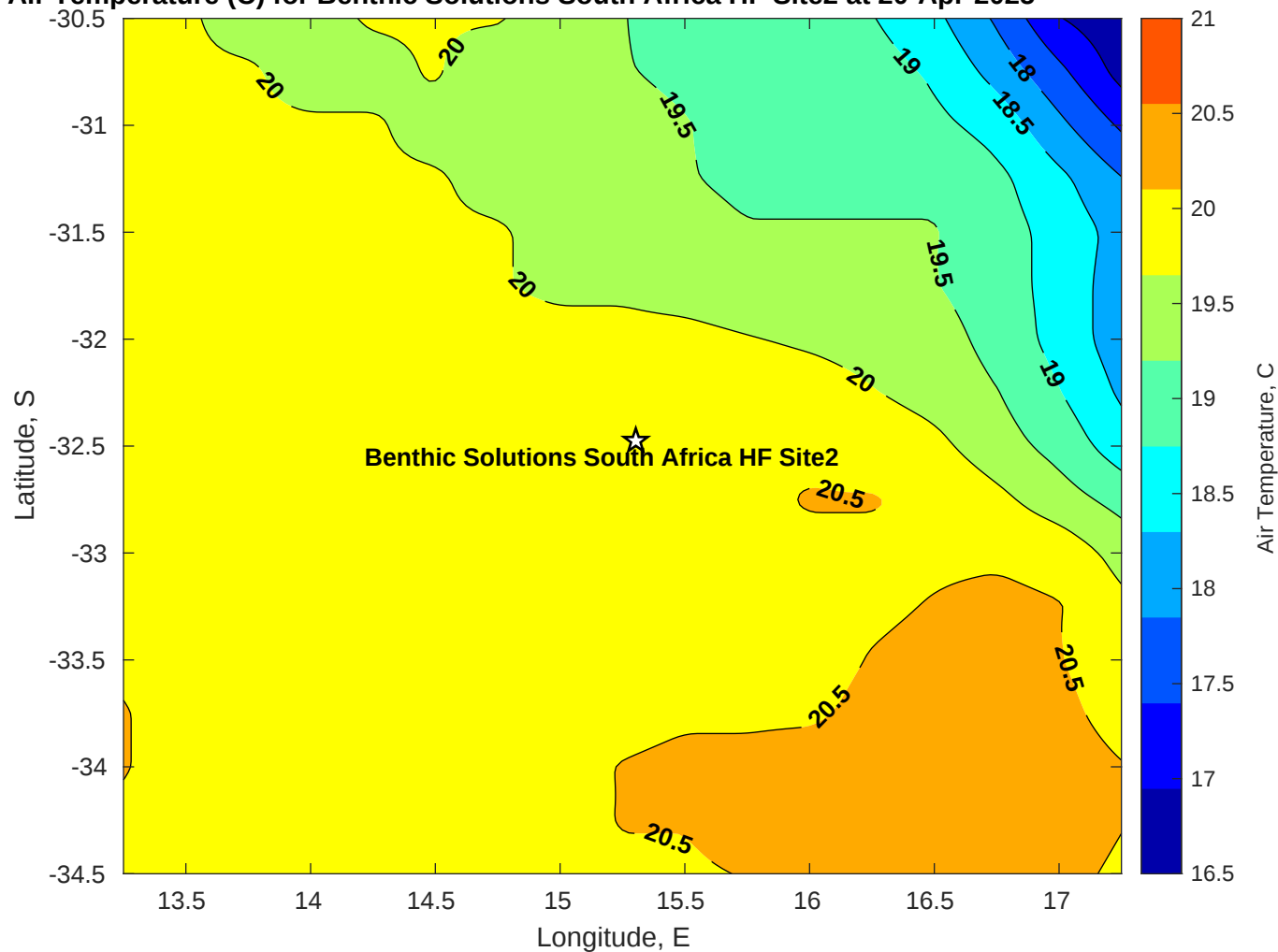
Air Temperature (C) for Benthic Solutions South Africa HF Site2 at 20-Apr-2025
