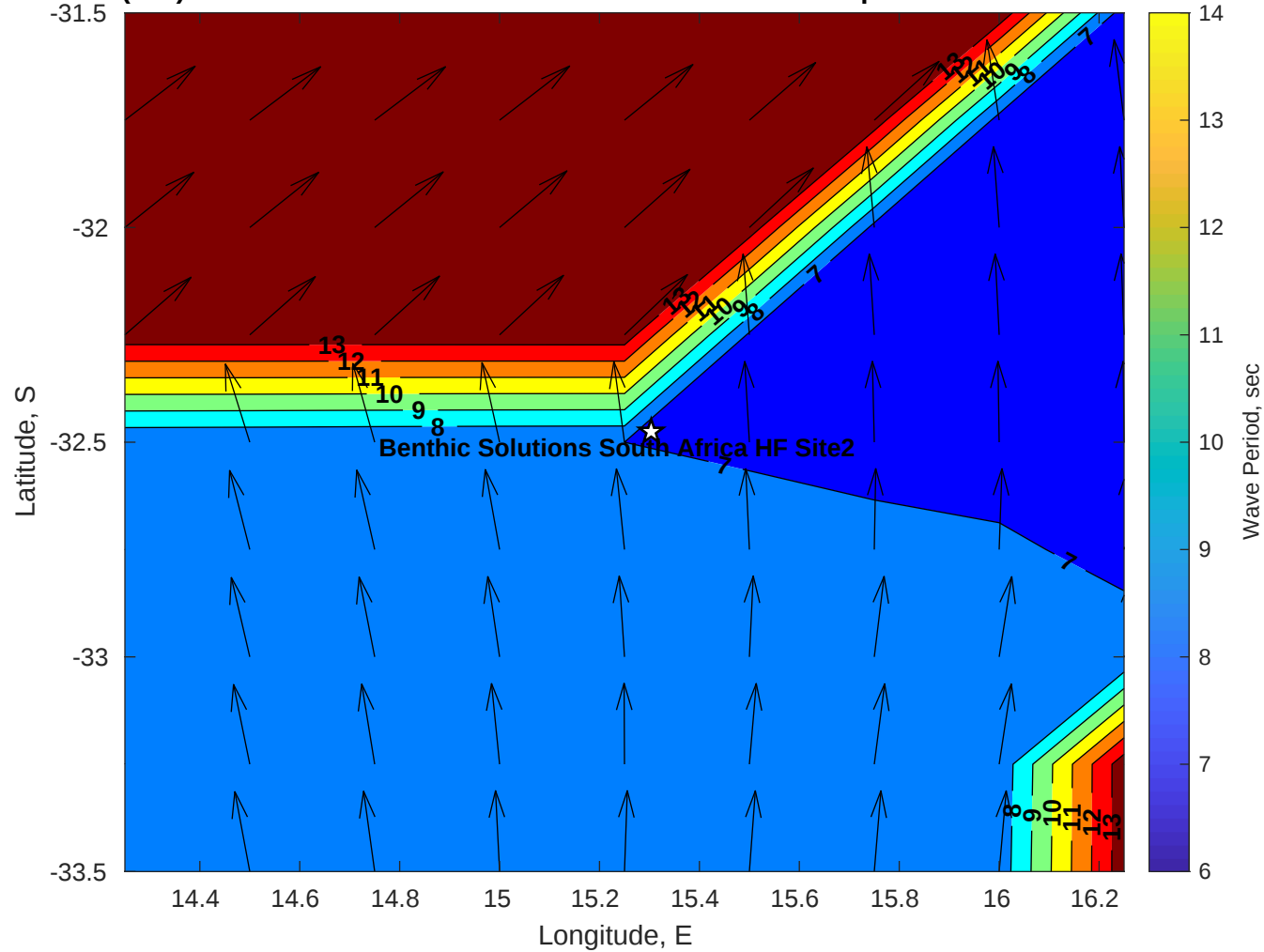
Wave Period (sec) for Benthic Solutions South Africa HF Site2 at 20-Apr-2025 09:00:00
