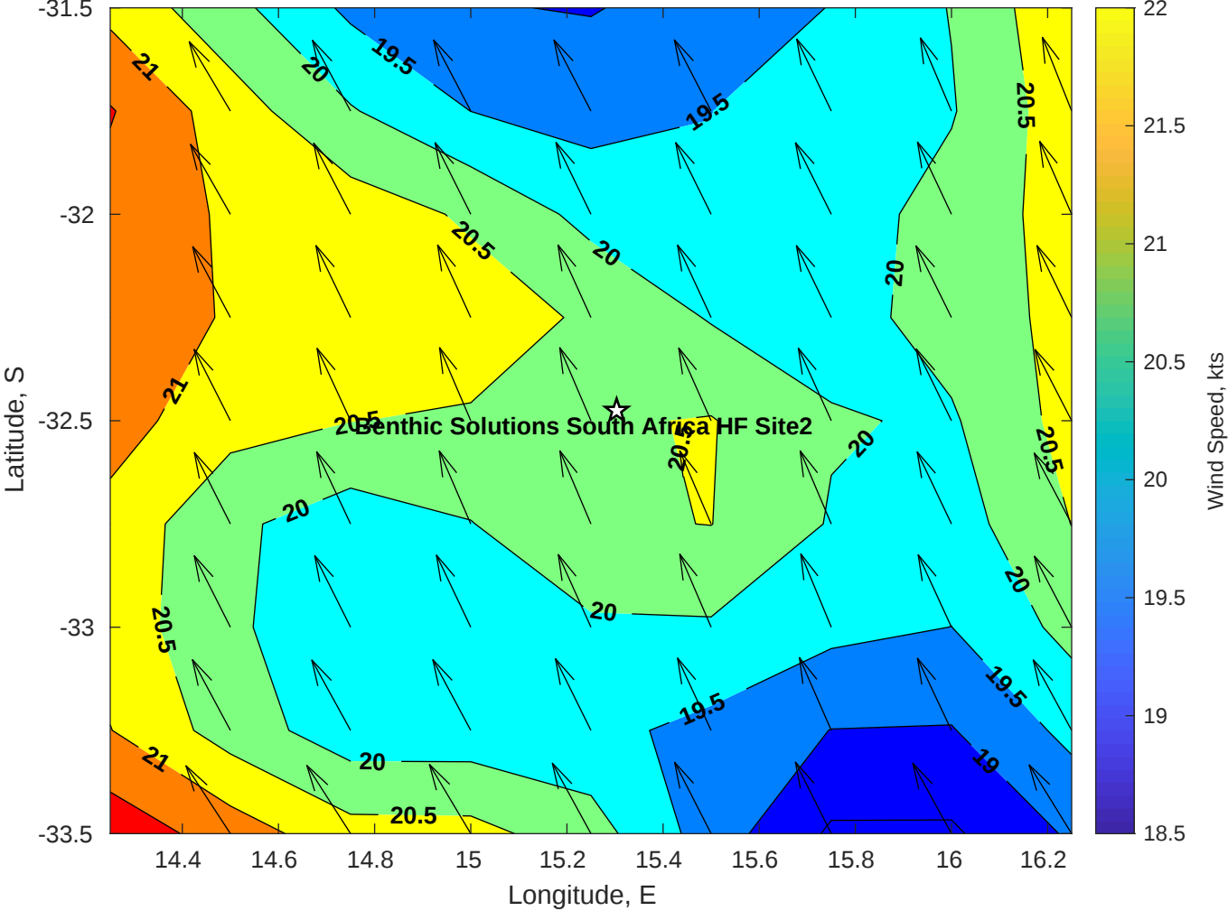
Winds (kts) for Benthic Solutions South Africa HF Site2 at 20-Apr-2025 09:00:00
