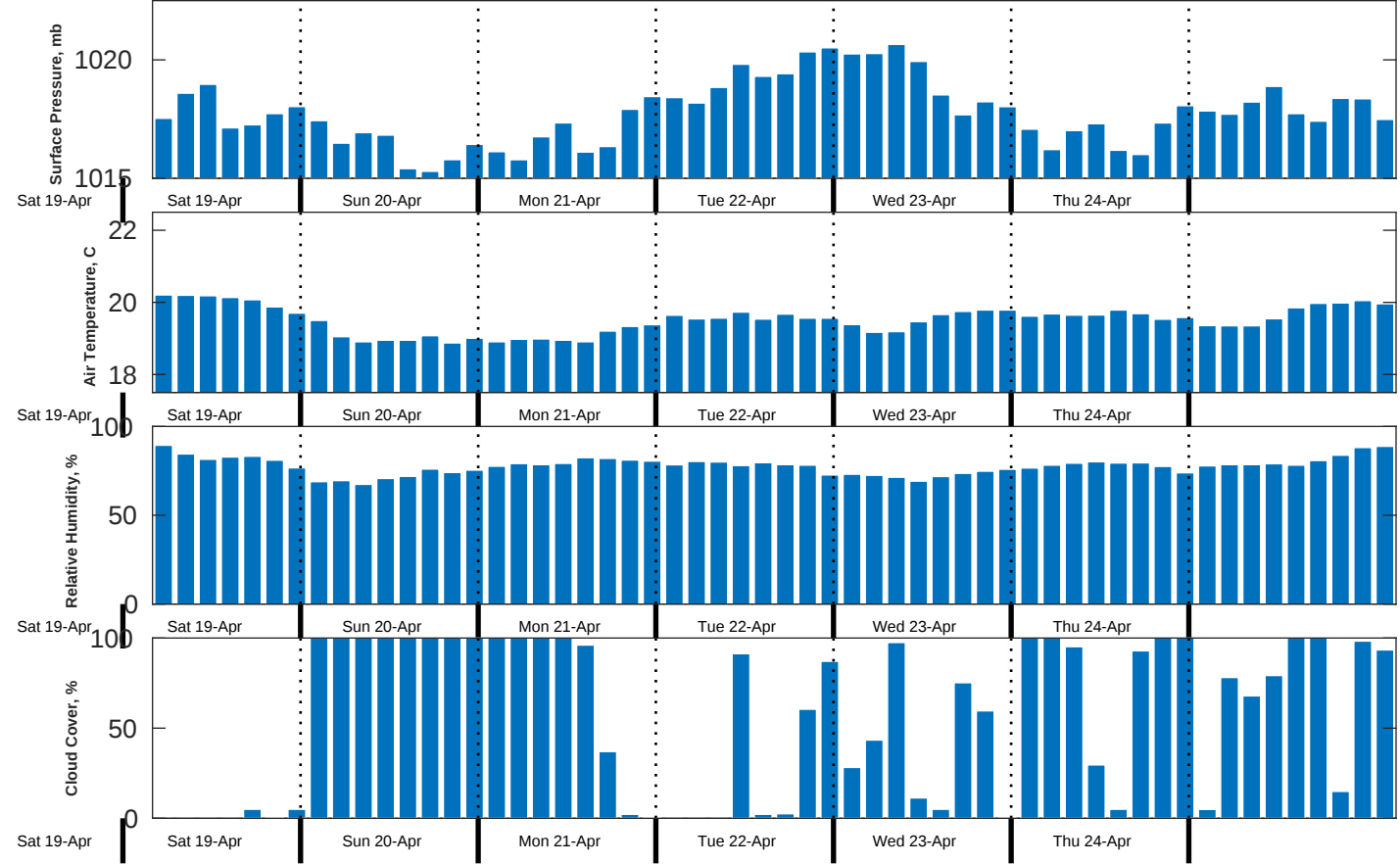
Met Forecast for Benthic Solutions South Africa HF Site2 from 20-Apr-2025 00:00:00 to 27-Apr-2025 00:00:00
