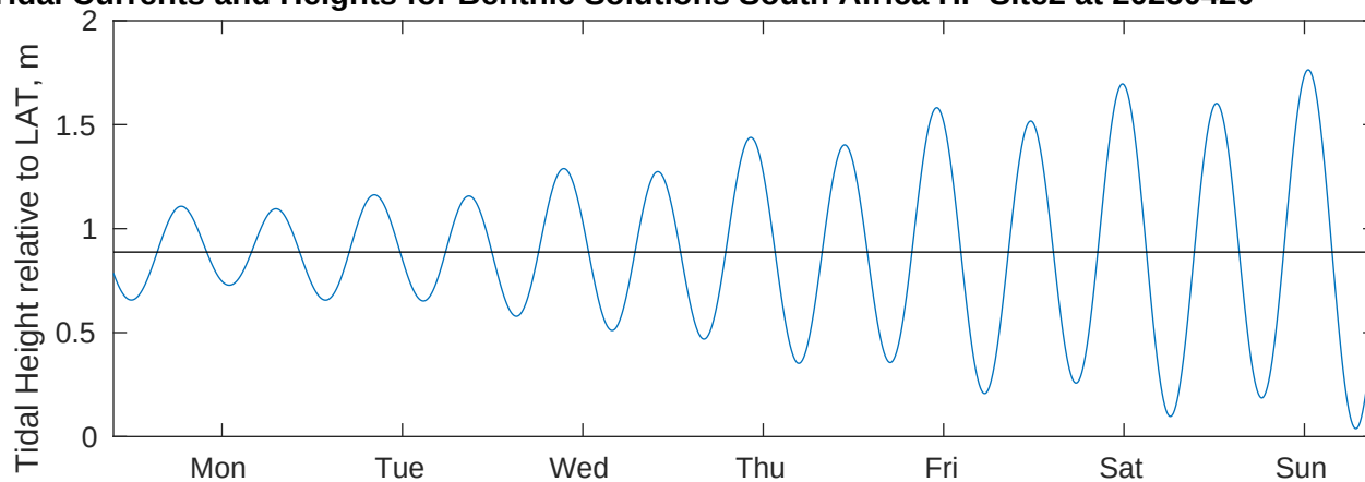
Tidal Currents and Heights for Benthic Solutions South Africa HF Site2 at 20250420
