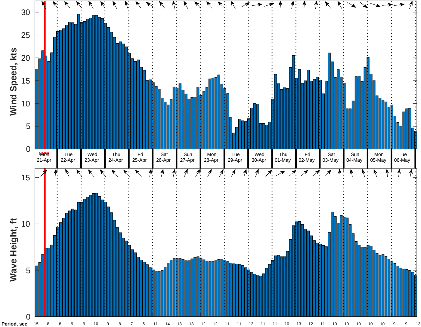
Wind & Wave Forecast for Benthic Solutions South Africa HF Site2 from 20-Apr-2025 02:00:00 to 06-May-2025 02:00:00
