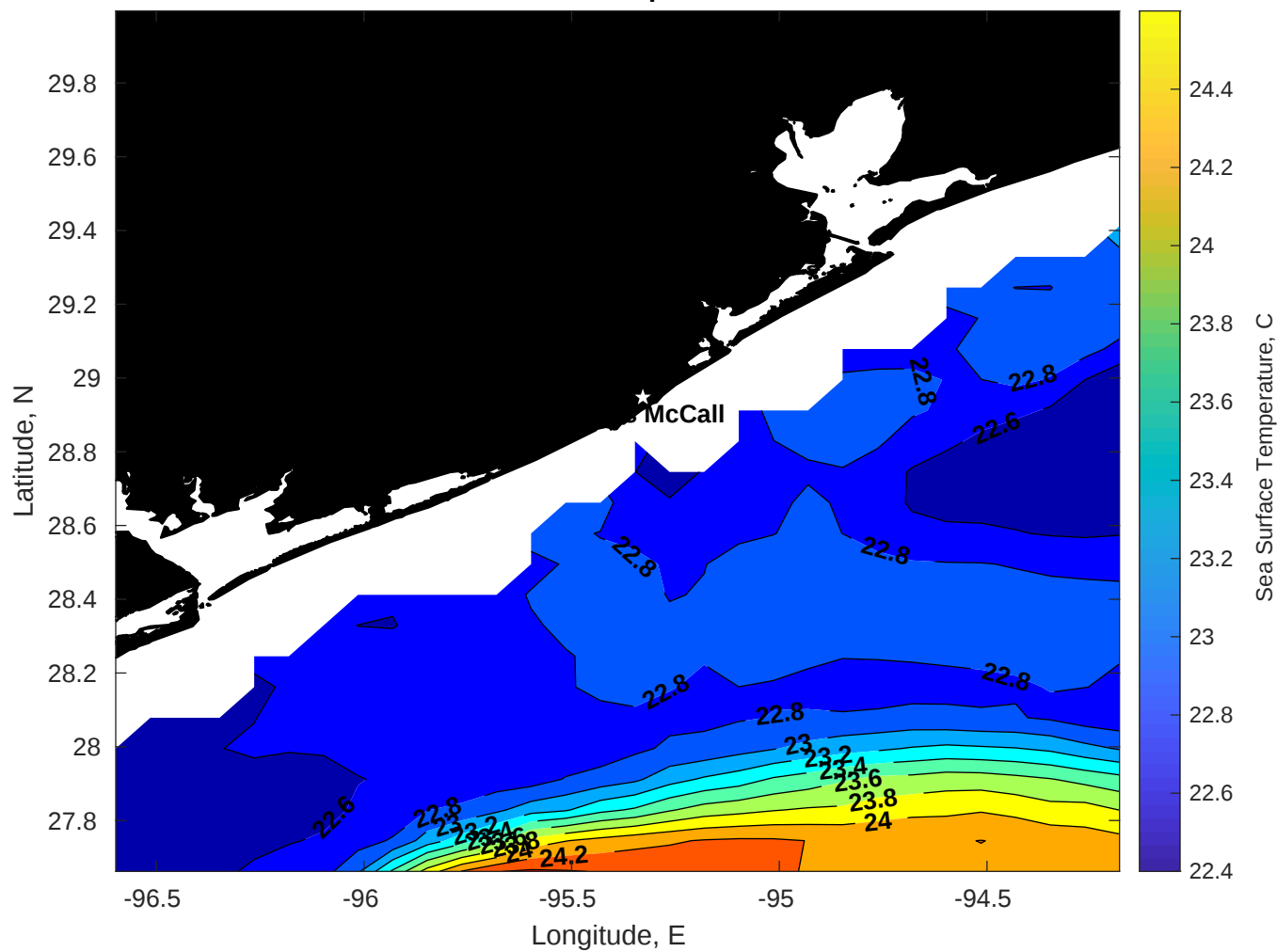
SST for Brooks McCall at 19-Apr-2025 00:00:00
