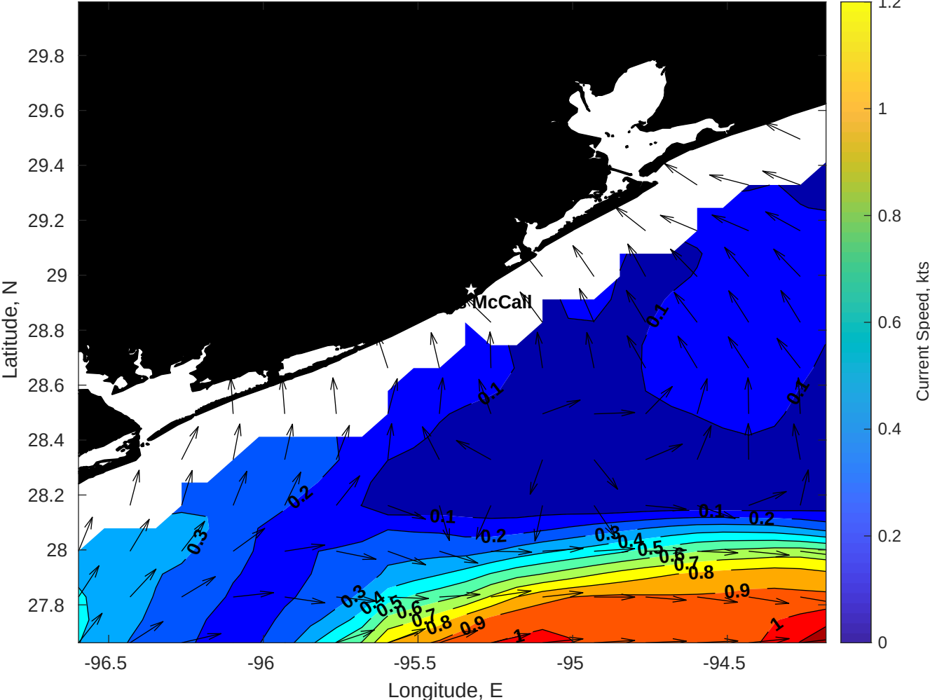
Surface Currents for Brooks McCall at 19-Apr-2025 00:00:00
