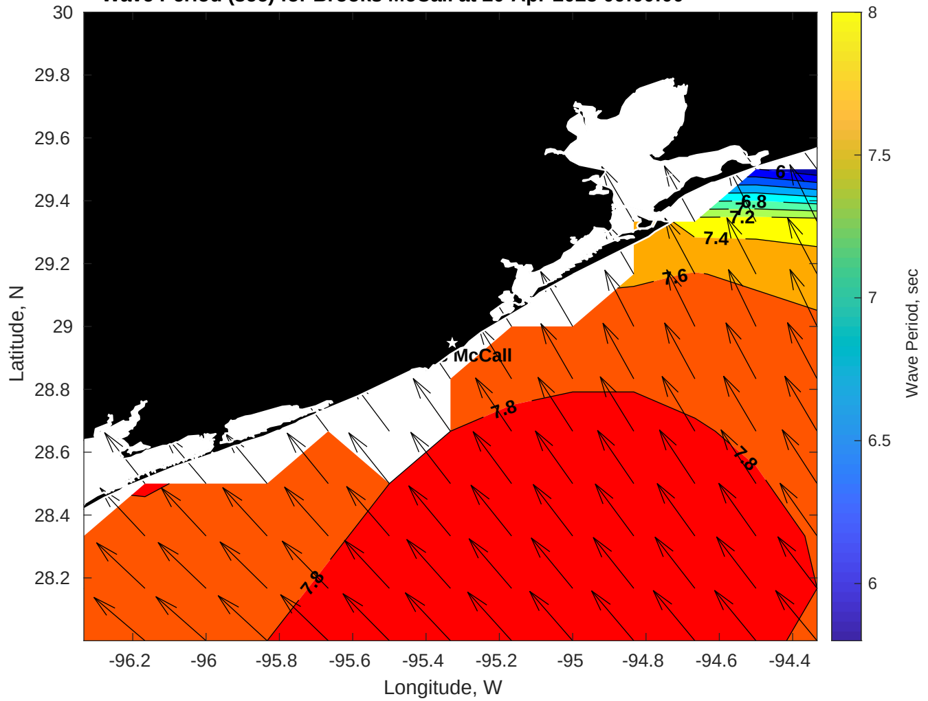
Wave Period (sec) for Brooks McCall at 20-Apr-2025 09:00:00
