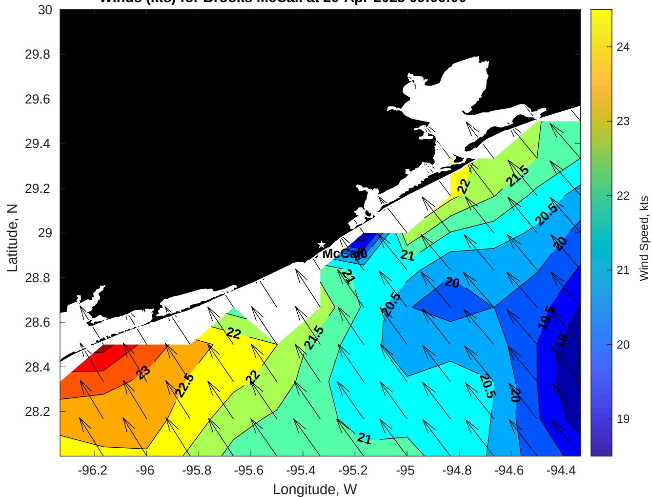
Winds (kts) for Brooks McCall at 20-Apr-2025 09:00:00
