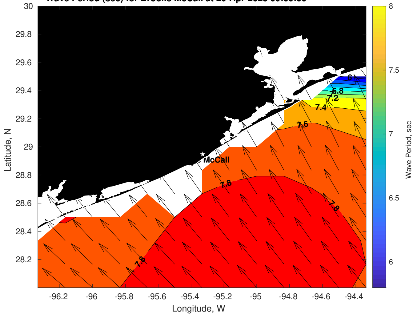
Wave Period (sec) for Brooks McCall at 20-Apr-2025 09:00:00
