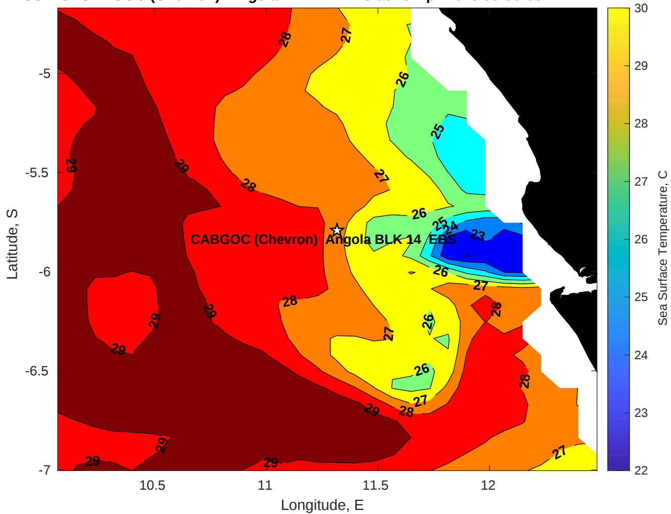
SST for CABGOC (Chevron) Angola BLK 14 EBS at 19-Apr-2025 00:00:00
