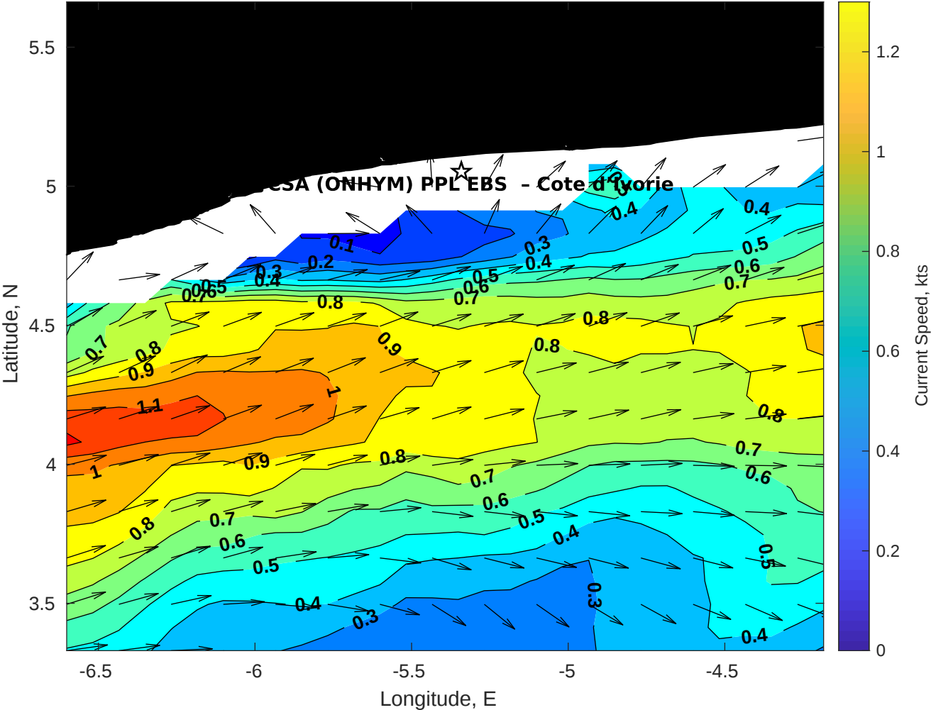
Surface Currents for CSA (ONHYM) PPL EBS - Cote d'Ivoire at 19-Apr-2025 00:00:00
